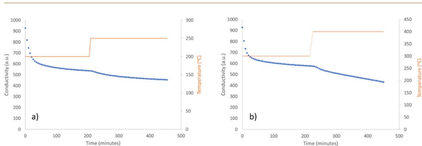
Fig. 18 Ammonia production reaction profiles of 'Co 3 MoN' reacted with 60 mL min -1 of 3 : 1 H 2 /N 2 (a) for 3 hours 25 minutes at 200 °C and 4 hours 5 minutes at 250 °C and (b) for 3 hours 35 minutes at 300 °C and 3 hours 45 minutes at 400 °C.
