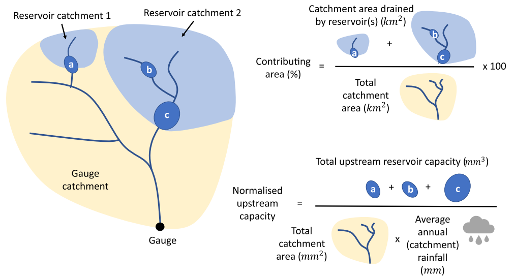
Figure 2. Schematic visualizing catchment descriptors and their equations for reservoir catchments. As demonstrated, the contributing area is the sum of reservoir catchments 1 and 2 divided by the total gauge catchment area, whilst the normalized upstream capacity is the sum of reservoirs 1, 2 and 3 capacities divided by the gauge area multiplied by the average annual (catchment) rainfall.
