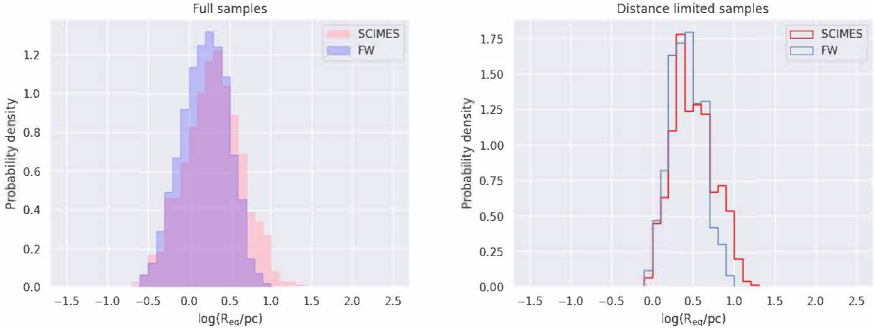
Figure 8. Distributions of equivalent radii in the SCIMES and FW segmentations (left panel). The right panels show the distributions for the distance-limited (8–12 kpc) samples.
