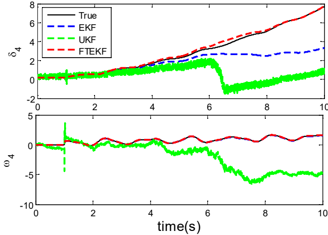
Fig. 6. Estimation results of \delta_4, \omega_4 for generator 4 of New England 39-bus system with partial missing measurements.
