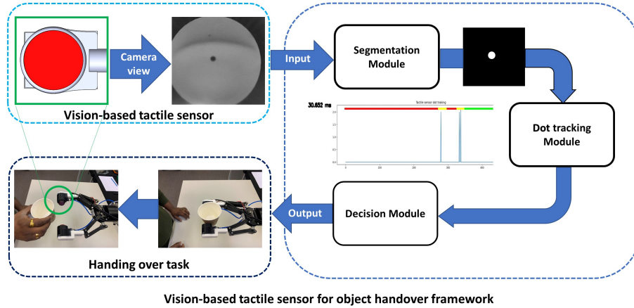
Fig. 1. Vision-based tactile sensor for handover framework
