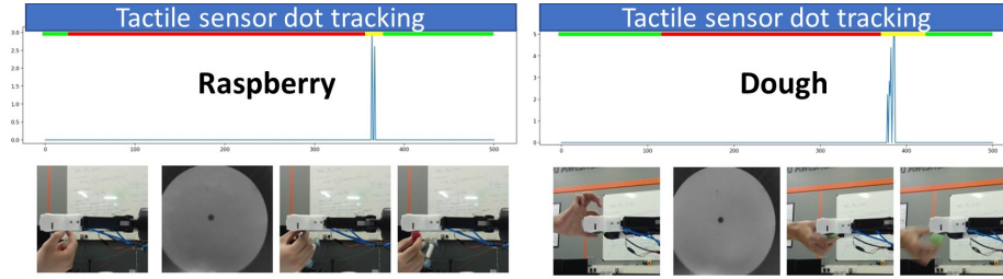
Fig. 3. A human and a robot are performing a handing-over task with raspberry (on the left) and dough (on the right) during the experiments. In the dot tracking plot, when the colour of the line is red, the gripper is closed. The yellow colour indicates that the user is trying to get the object. The green colour indicates that the gripper is open.
