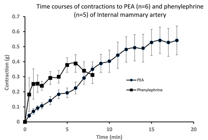
Fig. 4. Mean time courses for the contractions of human isolated internal mammary arteries to \beta -phenylethylamine (PEA) ( 3 \times 10^{-4} M, n = 6, ◆) and phenylephrine ( 10^{-5} M, n = 5, ■). Contractions are plotted as the mean \pm SEM increases in tension above baseline expressed as g tension.
