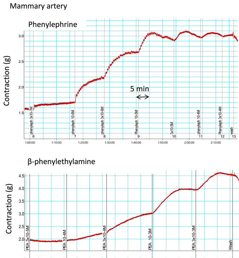
Fig. 1. Representative traces of contractions of human isolated internal mammary arteries to A. phenylephrine and B \beta -phenylethylamine (PEA). Phenylephrine and PEA were administered cumulatively in half logarithmic increments in concentration. The time scale for 5 min is shown and contractions are recorded in g tension.
