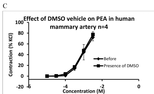
Fig. 5. Effect of prazosin (1 \mu\text{M} ) on contractions of human isolated mammary arteries to phenylephrine and \beta -phenylethylamine (PEA). Concentration-response curves are plotted as the mean \pm SEM increases in tension expressed as % of contraction to KCl 60 mM. Responses to A. phenylephrine (n = 4) and B. PEA (n = 5) are shown before ( \blacklozenge ) and in the presence of prazosin ( \blacklozenge ) and C. responses to PEA (n = 4) before ( \blacksquare ) and in the presence of dimethylsulfoxide (DMSO, 1 in 10 distilled water)( \blacksquare ).
