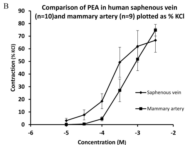
Fig. 2. Mean concentration-response curves for the contractions to \beta -phenylethylamine (PEA) compared in human internal mammary arteries (■)(n = 9) and saphenous veins (◆) (n = 10). Contractions are plotted as the mean \pm SEM increases in tension above baseline expressed as either A g tension or B percentage of the contraction to KCl (60 mM).
