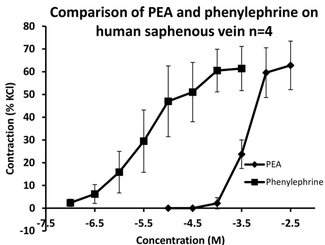
Fig. 3. Mean concentration-response curves (n = 4) for the contractions of human isolated saphenous vein to phenylephrine (■) and \beta -phenylethylamine (PEA)(◆). Contractions are plotted as the mean \pm SEM increases in tension above baseline expressed as percentage of contraction to KCl (60 mM).
