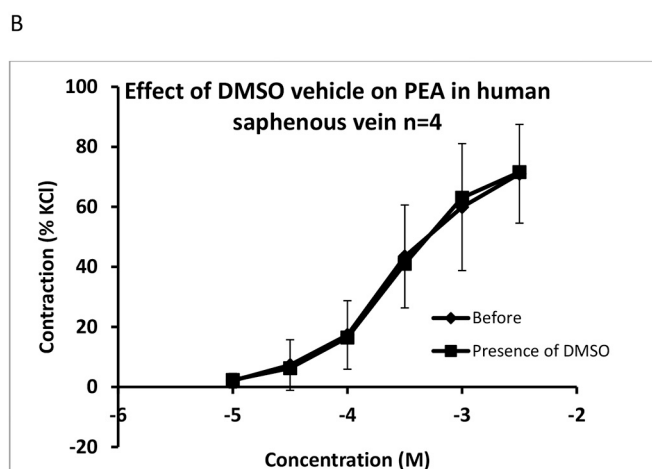
Fig. 6. Effect of prazosin (1 \mu\text{M} ) on contractions of human isolated saphenous veins to \beta -phenylethylamine (PEA). Concentration-response curves are plotted as the mean \pm SEM increases in tension expressed as % of contraction to KCl 60 mM. Responses to PEA are shown before ( \blacklozenge ) and in the presence of ( \blacksquare ) either A. prazosin (n = 6) or B. dimethylsulfoxide (DMSO, 1 in 10 distilled water)(n = 4).
