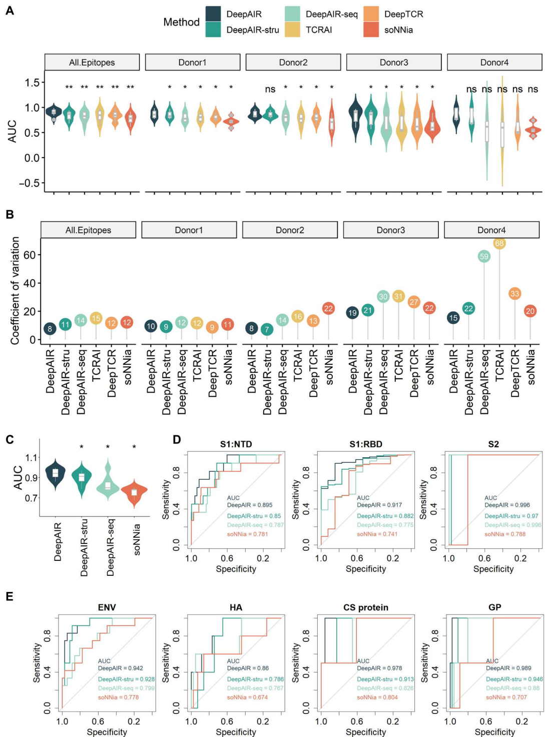
Fig. 4. Performance comparison between DeepAIR and state-of-the-art (SOTA) approaches for adaptive immune receptor (AIR)–antigen binding reactivity prediction.
