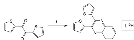
Scheme 4 Synthesis of 2,3-di(thiophen-2-yl)quinoxaline species, L 10H . Reagents and conditions: (i) 1,2-phenylenediamine, EtOH, AcOH, heat.
