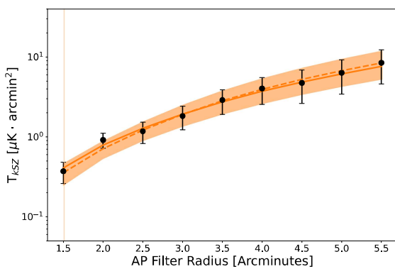
(b) The f150-only GNFW profile fit for the kSZ profile.
