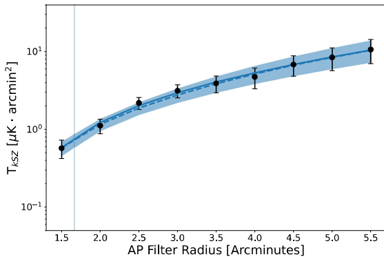
(a) The f090-only GNFW profile fit for the kSZ profile.
