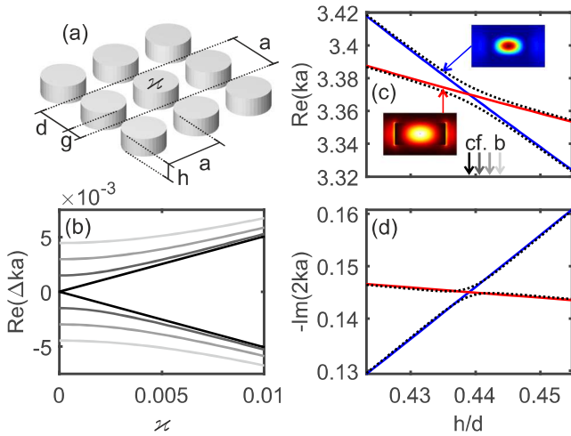
FIG. 4. (a) Schematic of a dielectric metasurface of high-index disks ( n_r = 3.5 ) with diameter d , period a , height h , and interparticle distance g . (b) Splitting of the wave number as a function of Pasteur parameter \varkappa . The splitting typically starts quadratically (gray lines), except for the case of quasidegeneracy (black lines), for which we have fine-tuned all parameters except for the refractive index of the disk. (c) Real and (d) imaginary parts of the wave numbers of the electric (red lines) and magnetic (blue lines) dipolar modes as a function of aspect ratio h/d for d = 505.1 nm, g = 222.8 nm, and a surrounding medium with n_r = 1.498 . The quasidegeneracy occurs for h = 221.7 nm. Insets in (c) show the resonant magnetic (top) and electric (bottom) fields of the magnetic and electric dipole mode, respectively, at h = 219.7 nm, while arrows mark the aspect ratios for the curves in (b).
