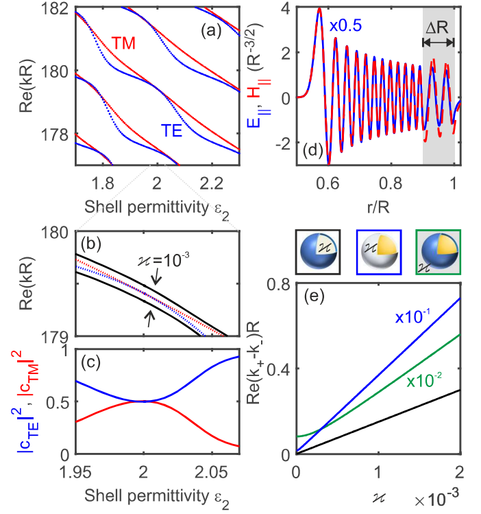
FIG. 2. (a) Real part of the wave numbers of l = 200 TE (blue) and TM (red) WGMs of a basis core-shell system, surrounded by vacuum, with \epsilon_1 = 4 in the core, shell thickness \Delta R = 0.1R , and system radius R , as functions of the shell permittivity \epsilon_2 . (b) Real part of the unperturbed (dashed lines) and perturbed (black solid lines) wave numbers, and (c) square moduli of the TE (blue) and TM (red) expansion coefficients in Eq. (6) of the perturbed lower branch as functions of \epsilon_2 , for a homogeneous chiral core perturbation of \chi = 10^{-3} . (d) Real part of the normalized electric field of TE (blue) and the imaginary part of the magnetic field of TM (red) WGMs of the core-shell system at \epsilon_2 = 2 . The wave numbers of the TE and TM modes are, respectively, k_1 R = 179.409265396 - 3.08 \times 10^{-7}i and k_2 R = 179.408443931 - 3.69 \times 10^{-7}i . (e) Real part of the wave-number splitting, k_+ - k_- , of the TE-TM quasidegenerate WGMs in (d), as a function of the Pasteur parameter \chi for chiral perturbations of the core (black), shell (blue), and vacuum (green), with the corresponding sketches of the system given on the top. Note that the blue curves in (d) and (e) and the green one in (e) have been rescaled for the sake of clarity. The actual results can be obtained by multiplying the curves with the same-color factors.
