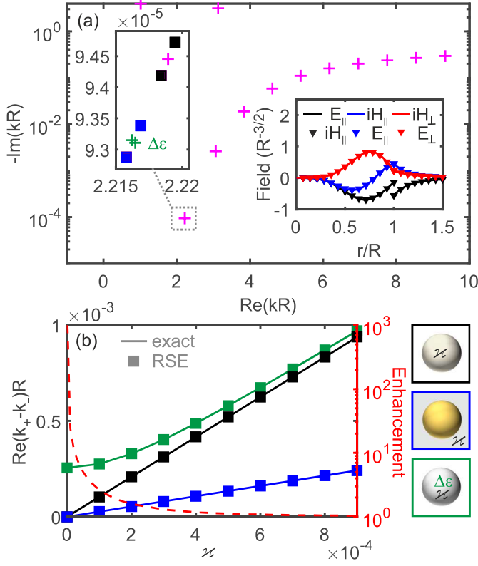
FIG. 1. (a) Wave numbers (magenta crosses) of strictly degenerate TE and TM RSs with angular momentum number l = 5 of a basis sphere of radius R and \epsilon = \mu = 4 , surrounded by vacuum. Right inset: radial dependence of tangential ( \parallel ) and normal ( \perp ) components of the normalized electric and magnetic fields of the fundamental WGM in TE (lines) and TM (triangles) polarizations, as defined in Eq. (28) of Ref. [29]. Left inset: Unperturbed degenerate (magenta cross) and perturbed split wave numbers of the fundamental WGM due to the dielectric ( \Delta\epsilon = 0.01 , green crosses), chiral ( \chi = 10^{-3} , black squares), and simultaneous dielectric and chiral ( \Delta\epsilon = 0.01 , \chi = 10^{-3} , blue squares) homogeneous perturbations of the basis sphere. (b) Real part of the wave-number splitting, k_+ - k_- (left axis), of the TE-TM degenerate fundamental WGM as a function of the Pasteur parameter \chi for chiral perturbations of the sphere (black), vacuum (blue), and sphere with an additional perturbation \Delta\epsilon = 0.01 (green), with the black-to-green chiral sensitivity enhancement factor (red, right axis, see main text for details) and the corresponding sketches of the system given on the right. Solid lines and squares are, respectively, the exact results and the RSE solution given by Eq. (7).
