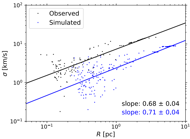
Figure A2. Same as Fig. 2, but using the self-variationalized simulation snapshot.
