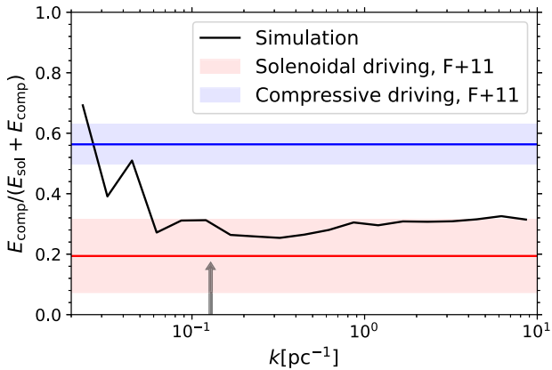
Figure A3. Same as Fig. 3, but using the self-variationalized simulation snapshot.
