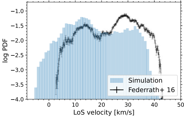
Figure A1. Same as Fig. 1, but using the self-variationalized simulation snapshot.
