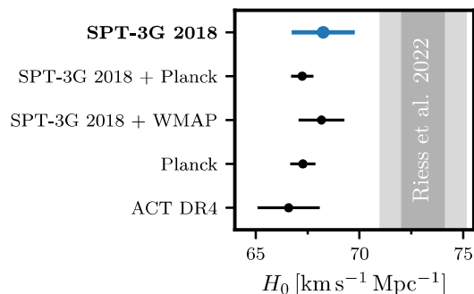
FIG. 10. Compilation of H_0 constraints from combinations of different CMB data sets assuming \Lambda CDM: SPT-3G 2018, Planck [1], WMAP [15], ACT DR4 [5]. The vertical gray band indicates the 2\sigma constraint from the most precise supernovae and distance ladder analysis [47]. SPT-3G 2018 data allow for a precision constraint on H_0 effectively independent from Planck data that deepens the Hubble tension.
