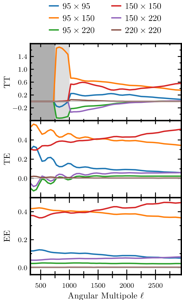
FIG. 6. Relative weight of each multifrequency spectrum entering the minimum-variance combination (diagonal elements of the mixing matrix). The gray shaded areas indicate the different \ell_{\text{min}} cuts of the TT spectra. Overall, the 95 \times 150 GHz and 150 \times 150 GHz spectra contribute the most weight. For TT data, all spectra bar the 220 \times 220 GHz band powers are non-negligible at intermediate \ell and the 95 \times 95 GHz TE data are important on large angular scales.
