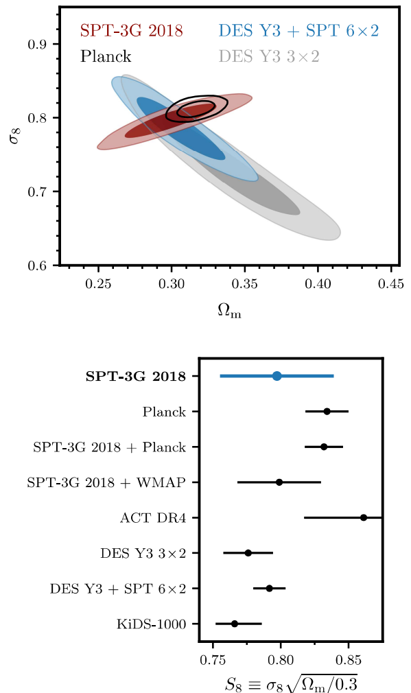
FIG. 11. Top panel: Constraints in the \sigma_8 vs. \Omega_m plane from SPT-3G 2018 (red), Planck (black line), a joint analysis of DES Y3 galaxy position and lensing data and SPT and Planck CMB lensing data ( 6\times 2 , blue) [54], and DES Y3 joint galaxy density and weak lensing data ( 3\times 2 , gray) [52]. The combined structure growth parameter, S_8 \equiv \sigma_8\sqrt{\Omega_m/0.3} , varies perpendicular to the degeneracy direction of the DES data.
