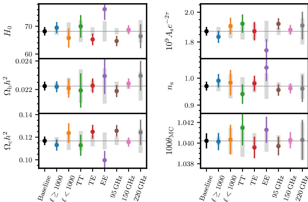
FIG. 3. Parameter constraints from the full SPT-3G 2018 TT/TE/EE data set (black points) and select subsets (coloured points as indicated) in \Lambda CDM. The grey boxes indicate the expected 1\sigma fluctuations between each subset and the full data set, taking the shared data into account. The observed shifts between subsets and the full data are consistent with statistical fluctuations. During the blind stage of this analysis, the parameter values along the vertical axes were not shown.
