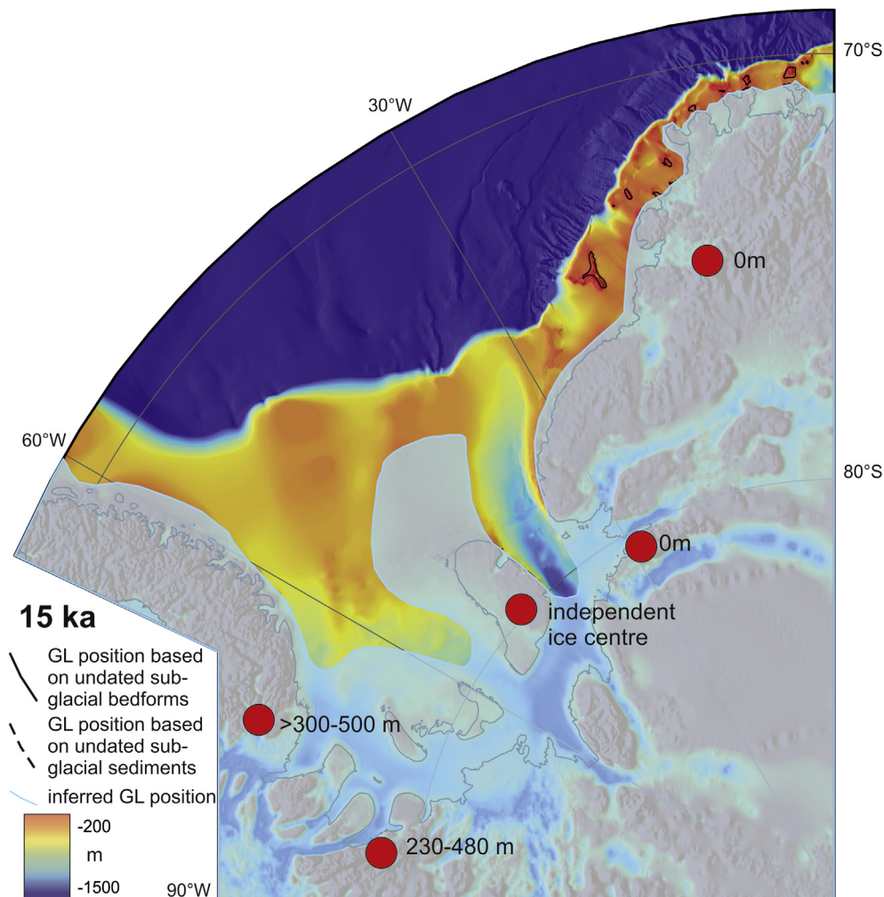
Fig. 9. Grounded ice-sheet extent in the Weddell Sea sector at 15 ka according to Scenario A.
