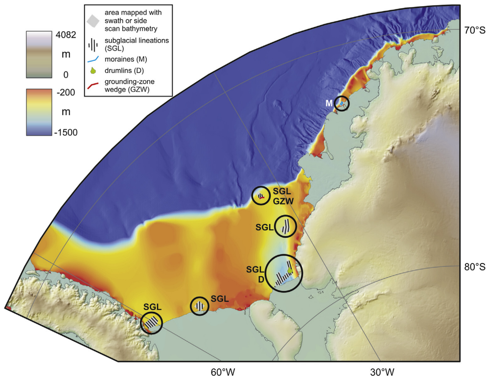
Fig. 2. Locations of subglacial bedforms in the Weddell Sea sector mapped by high-resolution bathymetry. The circles highlight the areas for which data have been published by Kristoffersen et al. (2000b), Larter et al. (2012) and Stolldorf et al. (2012).
