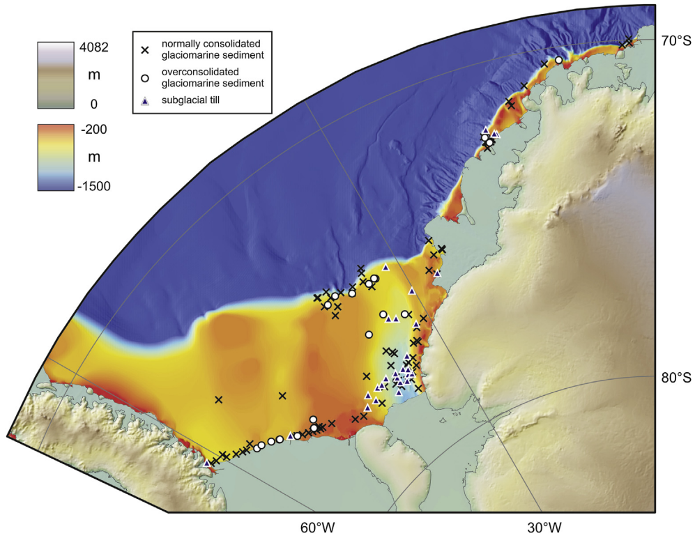
Fig. 3. Sites of marine sediment cores retrieved from the continental shelf and upper continental slope (above 1000 m water depth) in the Weddell Sea sector and distribution of normally consolidated glaciomarine sediments, over-compacted glaciomarine sediments and subglacial tills recovered in these cores (for details, see Supplementary Table 1).
