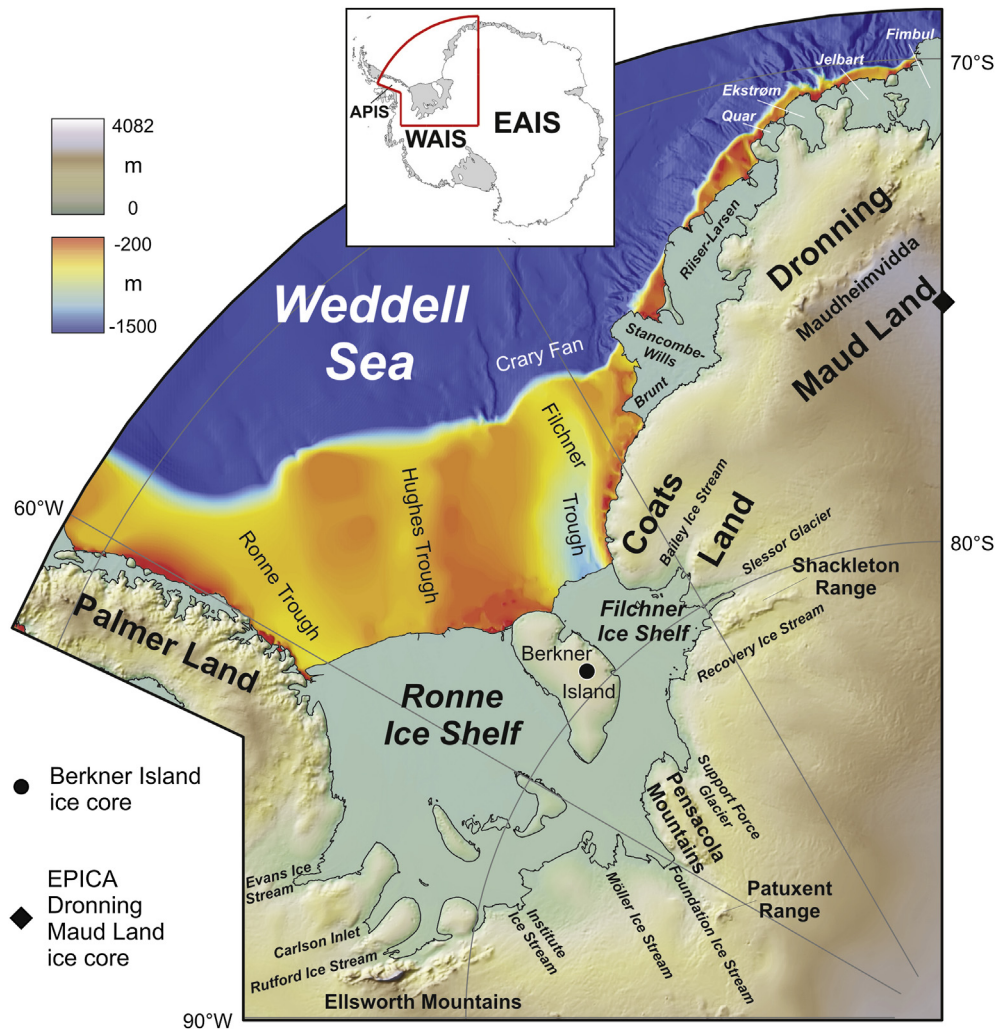
Fig. 1. Overview map over the Weddell Sea sector with shelf bathymetry and ice-sheet surface elevation (in metres above sea level) according to Bedmap2 (Fretwell et al., 2013) and the main physiographic and glaciological features. Ice shelves are displayed in light blue shading. Inset map shows the Weddell Sea sector outlined by the red line within the context of Antarctica, with ice shelves being displayed in grey shading (APIS: Antarctic Peninsula Ice Sheet, EAIS: East Antarctic Ice Sheet, WAIS: West Antarctic Ice Sheet).
