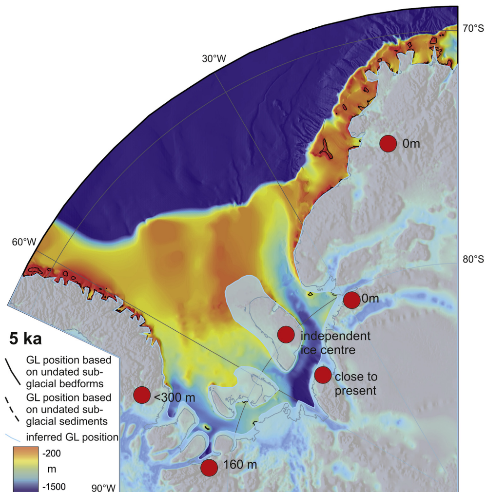
Fig. 11. Grounded ice-sheet extent in the Weddell Sea sector at 5 ka according to Scenario A.
