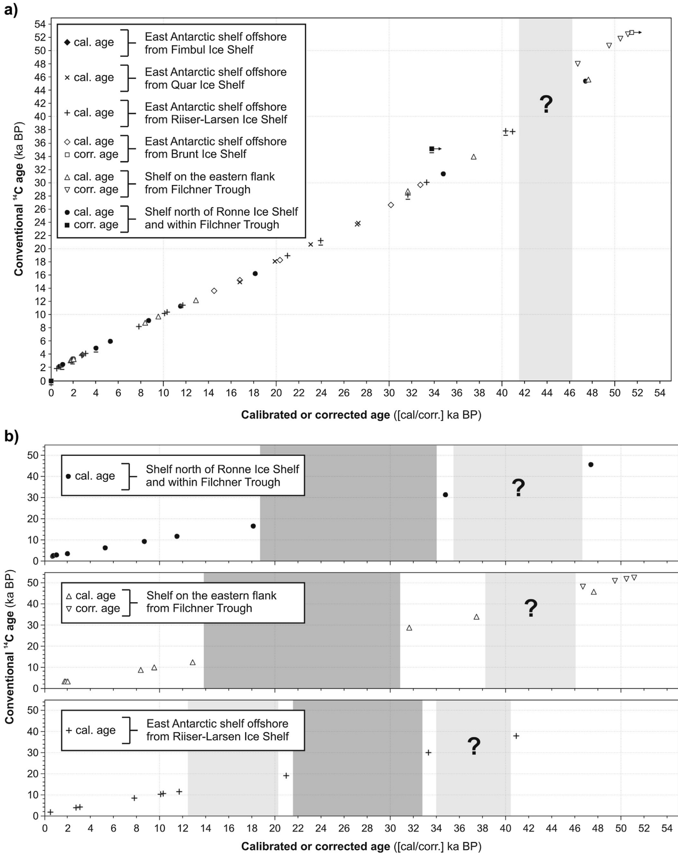
Fig. 5. Conventional radiocarbon dates versus calibrated (or corrected) radiocarbon ages from the cores displayed in Fig. 4 (for details see Supplementary Table 2). 5a: All ages grouped for different regions (note: Brunt Ice Shelf dates are exclusively from core 3-7-1, Quar Ice Shelf dates are exclusively from core 3-17-1 and the Fimbul Ice Shelf date is from core 206). Minimum ages are marked with arrows, and dates from cores recovered on the continental slope are underscored. Light grey shading indicates the time span of a
