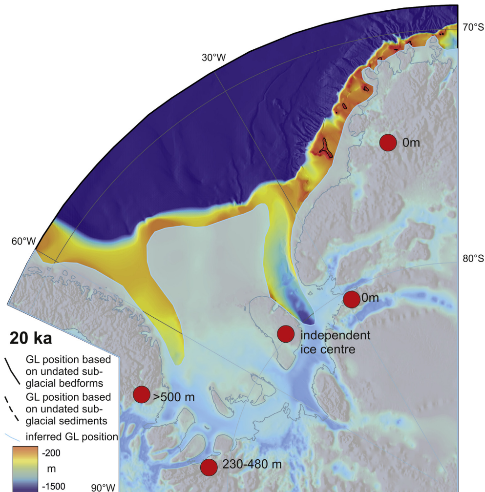
Fig. 8. Grounded ice-sheet extent in the Weddell Sea sector at 20 ka according to Scenario A (GL: grounding line).
