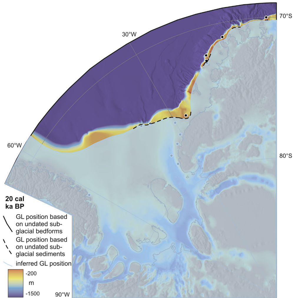
Fig. 13. Grounded ice-sheet extent in the Weddell Sea sector at 20 cal ka BP according to Scenario B.
