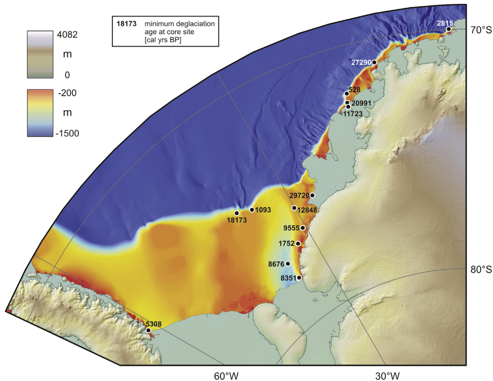
Fig. 7. Oldest calibrated radiocarbon ages obtained from cores offshore from the Brunt, Quar and Fimbul ice shelves (Fig. 5a) and calibrated radiocarbon ages constraining the termination of the most extended hiatuses observed north of the Filchner-Ronne and Riiser-Larsen ice shelves (see Fig. 5b). Only dates from cores collected from the continental shelf are displayed. These ages form the basis for the time-slice reconstructions according to Scenario B (see Figs. 12–16).
