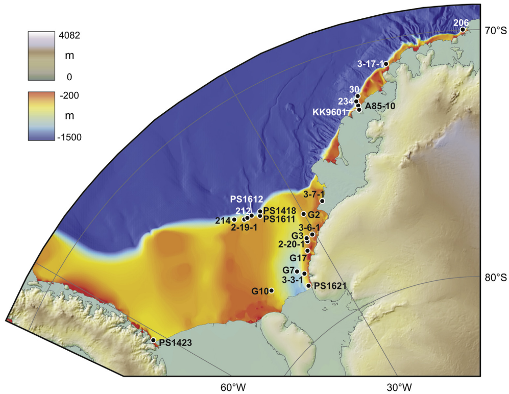
Fig. 4. Sites of marine sediment cores retrieved from the continental shelf and upper continental slope (above 1000 m water depth) in the Weddell Sea sector, for which radiometric and AMS radiocarbon dates have been published (for details, see Supplementary Table 2). Note that core PS1418 provided a core-top age only.
