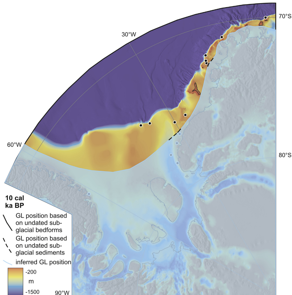
Fig. 15. Grounded ice-sheet extent in the Weddell Sea sector at 10 cal ka BP according to Scenario B.
