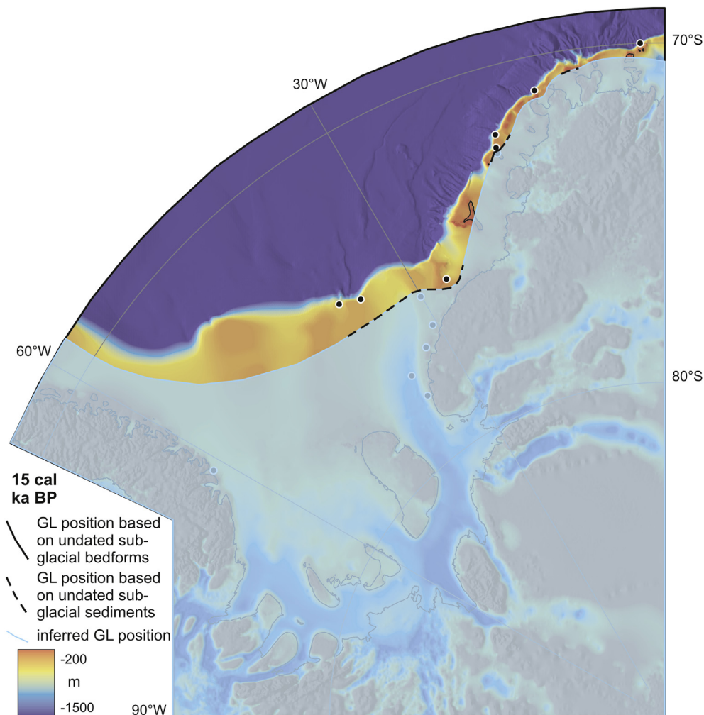
Fig. 14. Grounded ice-sheet extent in the Weddell Sea sector at 15 cal ka BP according to Scenario B.
