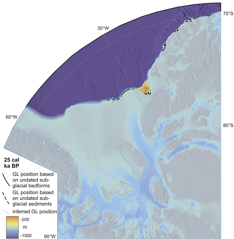
Fig. 12. Grounded ice-sheet extent in the Weddell Sea sector at 25 cal ka BP according to Scenario B. The position of the grounding line (GL) was reconstructed using the ages displayed in Fig. 7. The different certainty levels for the GL indicate whether its position is (i) constrained by nearby subglacial bedforms of unknown age (Fig. 2), (ii) constrained by nearby sediment cores that recovered subglacial/over-consolidated deposits of unknown age (Fig. 3), or (iii) simply inferred.
