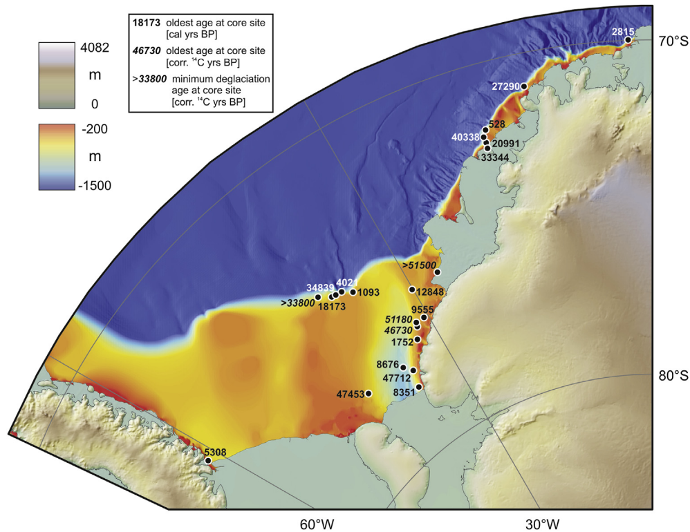
Fig. 6. Oldest calibrated (or corrected) radiocarbon ages from the cores displayed in Fig. 4 (except from core PS1418).
