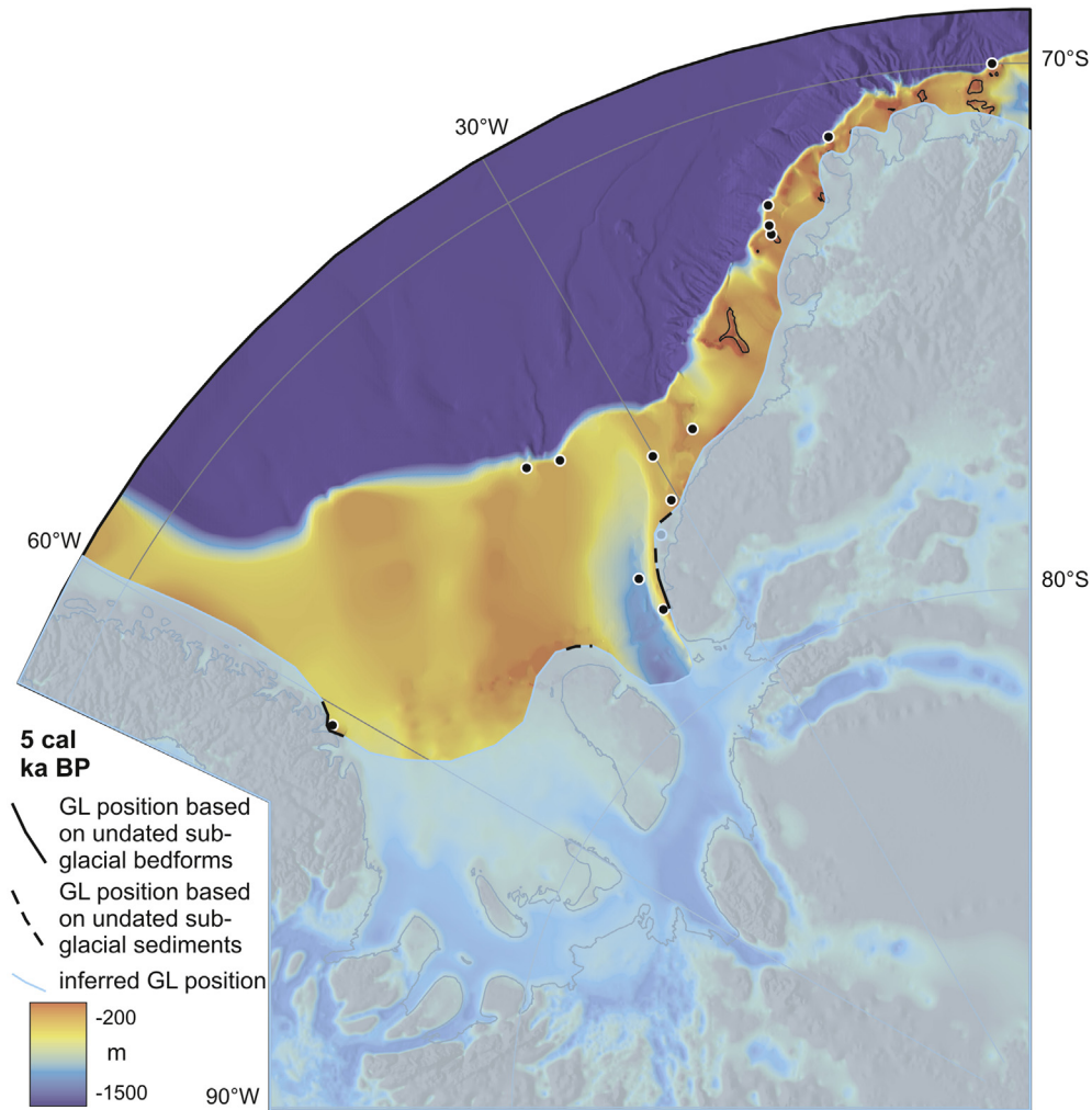
Fig. 16. Grounded ice-sheet extent in the Weddell Sea sector at 5 cal ka BP according to Scenario B.
