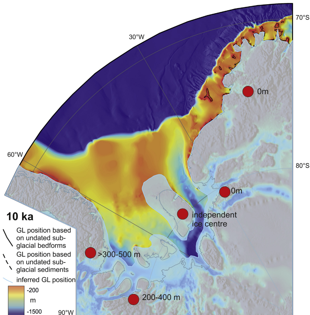
Fig. 10. Grounded ice-sheet extent in the Weddell Sea sector at 10 ka according to Scenario A.
