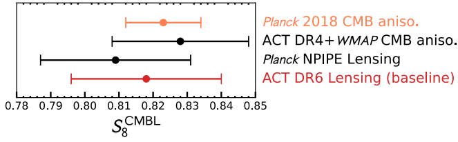
Figure 28. Marginalized posteriors for S_8^{\text{CMBL}} from ACT DR6 lensing (red). We also show the constraints from Planck NPIPE lensing and the early-universe extrapolation from CMB anisotropy measurements of ACT DR4 + WMAP and Planck 2018.
