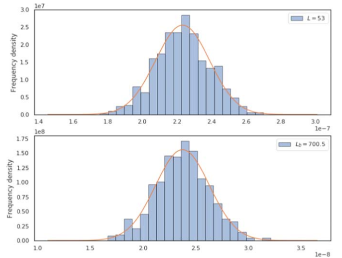
Figure 41. To test that a Gaussian likelihood for the lensing power spectrum bandpowers is sufficient, we plot histograms of the distribution of C_L^{\phi\phi} bandpowers obtained from simulations for a bin with L_B = 53 (top panel) and L_B = 700.5 (bottom panel). In both cases, the distribution of the bandpowers closely follows a Gaussian distribution with the expected properties (i.e., a mean and width given by the bandpower mean and standard deviation). No evidence for departures from Gaussianity is found.
