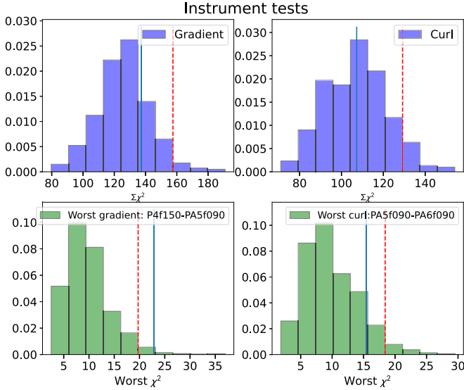
Figure 11. Same as Figure 9, but for null tests related to instrument systematics. These include the map-level array-difference tests described in Section 6.4.5 and the PWV and season-difference null tests introduced in Section 6.5.11. We again find no evidence for systematic effects in our data.
