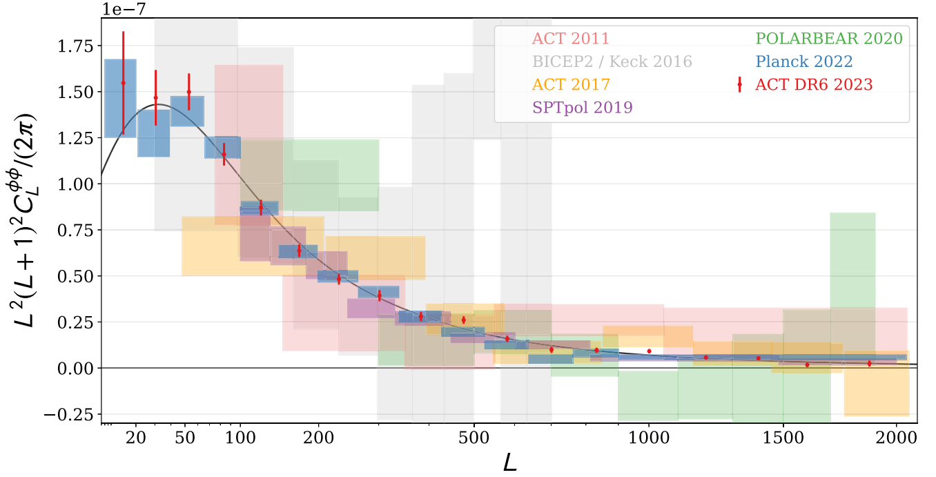
Figure 26. Compilation of CMB lensing power spectrum measurements, with our results shown as red data points. The CMB lensing power spectrum presented in this paper represents (along with Planck NPIPE, which reaches similar precision) the highest-S/N lensing spectrum measured to date.
