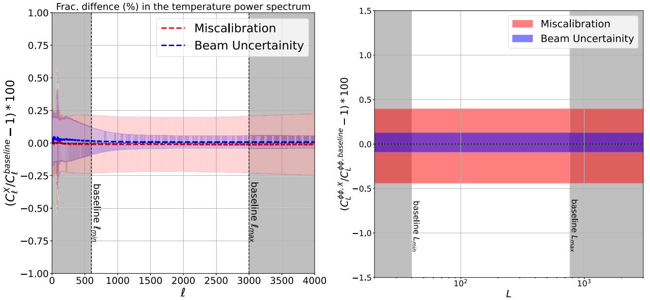
Figure 37. Left: mean and 1\sigma confidence intervals of the reprocessed coadded temperature power spectrum compared to the baseline. The scatter is due to uncertainties in calibration factors (shown in red) and instrument beams (shown in blue). The confidence intervals are computed using the 100 MC samples of calibration and beams applied to raw maps processed in the same way as the baseline. The grayed-out regions are outside of the baseline analysis range. Right: similar to the left panel, but for the lensing power spectrum. This is computed using the same 100 samples but with the fractional error in the CMB power spectrum propagated to the lensing power spectrum with the approximation \Delta \ln C_L^{\phi\phi} \approx 2\Delta \ln \tilde{C}_l discussed in the text. The grayed-out regions are outside of the baseline analysis range.
