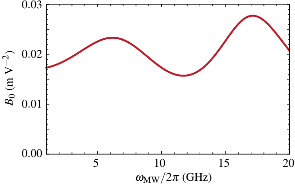
FIG. 4. Predicted dependence of the Kerr coefficient B_0 on microwave frequency \omega_{\text{MW}} at excitation energy E = 2.171411 eV.
