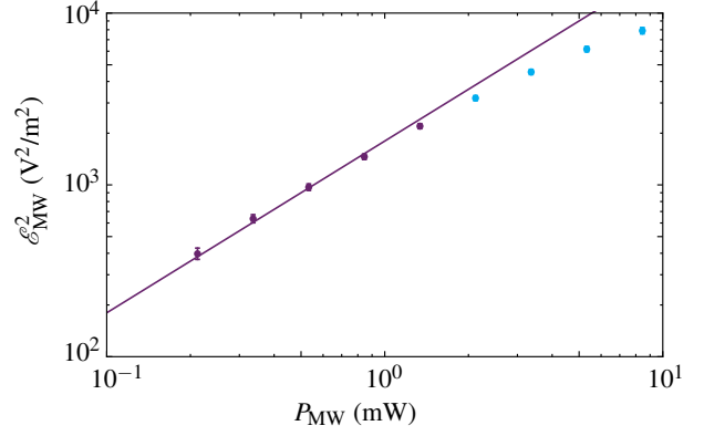
FIG. 5. Square of the fitted microwave electric field strength \mathcal{E}_{\text{MW}} versus microwave power applied at the input port of the stripline (output terminated at 50 Ohms) P_{\text{MW}} . By fitting the region where the model is valid (purple points) with a linear trend (purple line) the electric field calibration is extracted.
