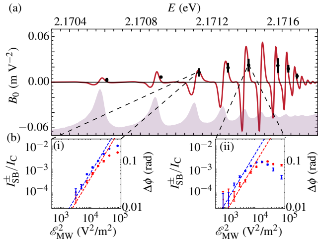
FIG. 3. (a) Predicted (solid line) and measured (points) Kerr coefficient vs excitation energy E . Shaded area shows exciton spectrum from n = 8 upwards for reference. (b) I_{\text{SB}}/I_C vs \mathcal{E}_{\text{MW}}^2 for positive frequency (blue) and negative frequency (red) sidebands. Right-hand axis gives the corresponding phase shift.
