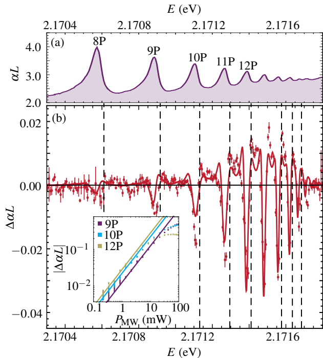
FIG. 2. (a) Rydberg series of exciton absorption lines. (b) Measured (red points) and predicted (solid line) change in absorption, \Delta\alpha L at \mathcal{E}_{\text{MW}} = 38 V/m. Dashed lines indicate the zero crossings used to extract the Kerr coefficient. Inset shows |\Delta\alpha L| versus microwave power P_{\text{MW}} at the n = 9, 10, 12\text{P} resonances. Solid lines are fits to the linear region.
