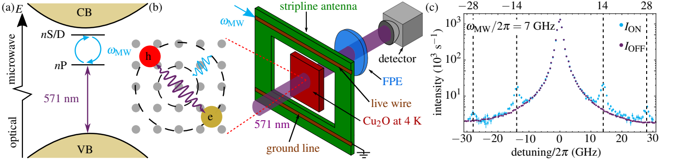
FIG. 1. (a) Excitons are created in state nP via laser excitation at \lambda \approx 571 nm. A microwave field at frequency \omega_{\text{MW}} couples odd- and even-parity exciton states. The exciton wavefunction spans many lattice sites giving rise to a large dipole moment. (b) Excitons are created in a thin slab of \text{Cu}_2\text{O} located between the conductors of a microwave stripline. The transmitted light is filtered with a Fabry-Pérot etalon (FPE) and sent to a detector. (c) Example spectrum of the transmitted light for E = hc/\lambda = 2.170927 eV and \mathcal{E}_{\text{MW}} = 640 V/m, showing an array of sidebands at \pm 2\omega_{\text{MW}}/(2\pi); \pm 4\omega_{\text{MW}}/(2\pi) when microwaves are applied ( I_{\text{ON}} ).
