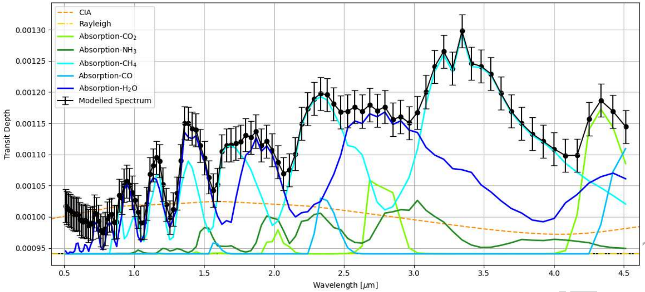
Figure 2: Forward modelled spectrum for candidate HD 106315 c, binned to R=50 from 0.5–4.5 \mu\text{m} . Molecular absorption components are shown at the binned resolution of the final spectrum. Also shown are the total contributions to the final spectrum from CIA (between \text{H}_2\text{-H}_2 and \text{H}_2\text{-He} ) and Rayleigh scattering (all atmospheric molecules), with the final spectrum shown in black.
