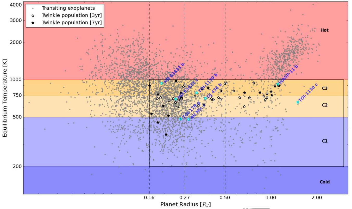
Figure 3: Population of known exoplanets [NASA Exoplanet Archive, accessed 18/05/23], overlain by candidates targeted by this study for the primary 3-yr and extended 7-year Twinkle exoplanet surveys. The different temperature regimes are indicated: Hot, C3, C2, C1 and cold. C1, C2 and C3 are three sub-categories of the "cool" regime. The bounded region indicated the parameter space of cool gaseous planets as defined in this paper. The equilibrium temperatures shown for Twinkle 3- and 7-year mission candidates are obtained from methodologies outlined in Edwards et al. (2019b) and used in the TwinkleRad database. For all other planets, the equilibrium temperatures shown are obtained from the NASA archive where available or otherwise calculated from stellar and orbital parameters (assuming an albedo of 0.3).
