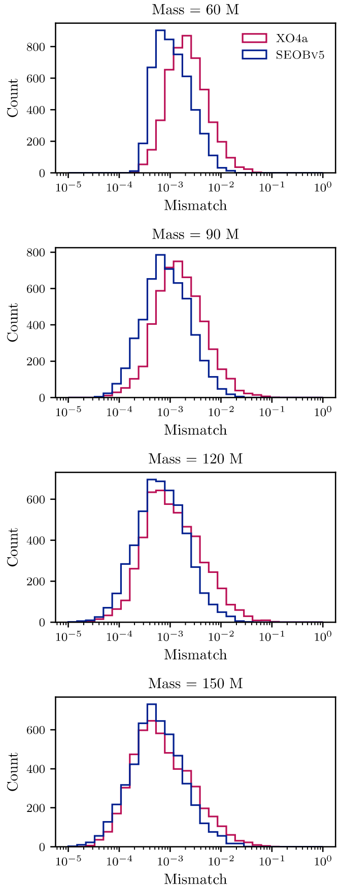
FIG. 10. Mismatches between the \ell = 2 multipoles in the J frame of NRSUR, XO4a and SEOBv5. Considered 1024 two-spin configurations at four different total masses \{60, 90, 120, 150\}M_{\odot} and five different inclinations \{0, \pi/3, \pi/2, 2\pi/3, \pi\} rad.
