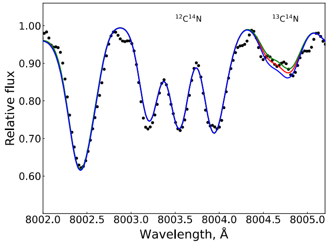
Fig. 3. Examples of fits to the ^{12}C^{14}N and ^{13}C^{14}N molecular lines in a spectrum of KIC4457200. The middle line represents the best fit for ^{12}C/^{13}C = 12 , whereas the other two lines indicate \pm 2 in the ^{12}C/^{13}C ratio.
