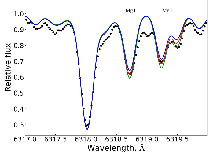
Fig. 4. Example of fits to the magnesium lines for KIC4457200. The middle line represents the best fit for [Mg/H] = 0.22 , whereas the other two lines indicate \pm 0.10 dex for the magnesium abundance.
