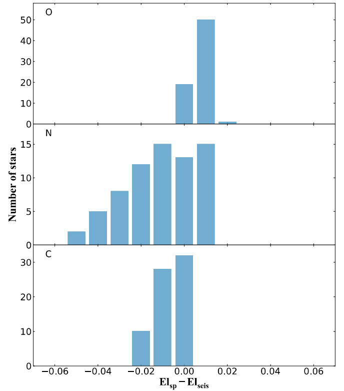
Fig. 5. Differences in abundances of C, N, and O derived using the spectroscopic and asteroseismic atmospheric parameters.
