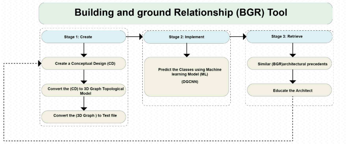
Figure 6: The workflow of the BGR tool
