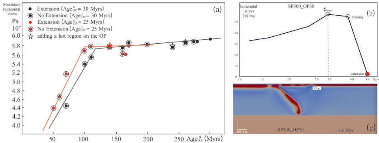
Figure 11. (a) Maximum vertically averaged horizontal stress ( \sigma_{hmax} ) over OP thickness (from the surface to the OP bottom, 50 km depth when the Age OP 0 is 30 Myrs and 45 km depth when the Age OP 0 is 25 Myrs which was defined by the temperature contour of 1300K.) vs. Age OP 0 . The stars mark the models which have a hot region on the OP. (b) Depicts the time evolution of vertically averaged horizontal stress ( \sigma_h ) and (c) identifies the specific location (in the viscosity field) where the stress in panel (b) is calculated. (b) and (c) are both from model SP300_OP30. A positive stress value means extensional.
