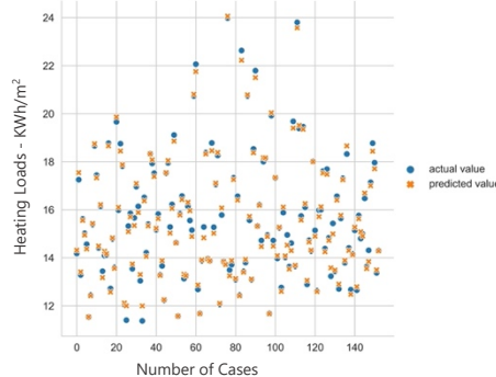
Figure 8 Actual versus predicted values for randomly selected test cases.
