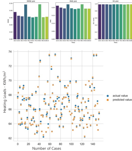
Figure 14 Graph shows actual versus predicted values for randomly selected test cases.
