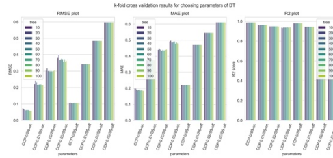
Figure 6 Results of hyperparameter tuning in RF.
