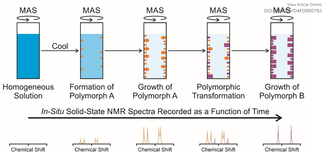
Figure 1. Schematic of the in-situ solid-state NMR strategy to study crystallization processes, showing a crystallization system in which a meta-stable polymorph (polymorph A; orange) is formed initially, followed by transformation to produce a more stable polymorph (polymorph B; purple), with polymorphs A and B distinguished on the basis of their solid-state NMR spectra.
