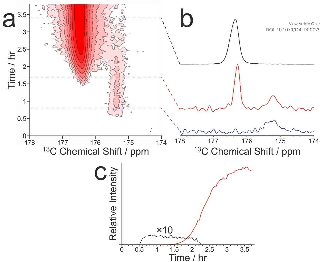
Figure 3. (a) Intensity contour plot showing the in-situ ^1\text{H}\rightarrow^{13}\text{C} CP NMR spectra recorded as a function of time during crystallization of 1- ^{13}\text{C} -glycine from water-glycerol at -10^\circ\text{C} . Contours are based on a log scale with a factor of 2 between adjacent contours. The isotropic peak due to the \beta polymorph is at ca. 175.5 ppm, and the isotropic peak due to the \alpha polymorph is at ca. 176.5 ppm. (b) Selected spectra from (a) recorded at 0.8 hr (blue), 1.7 hr (red) and 3.4 hr (black). (c) Relative intensities of the signals due to the \beta polymorph (black) and \alpha polymorph (red) as a function of time during the crystallization process.
