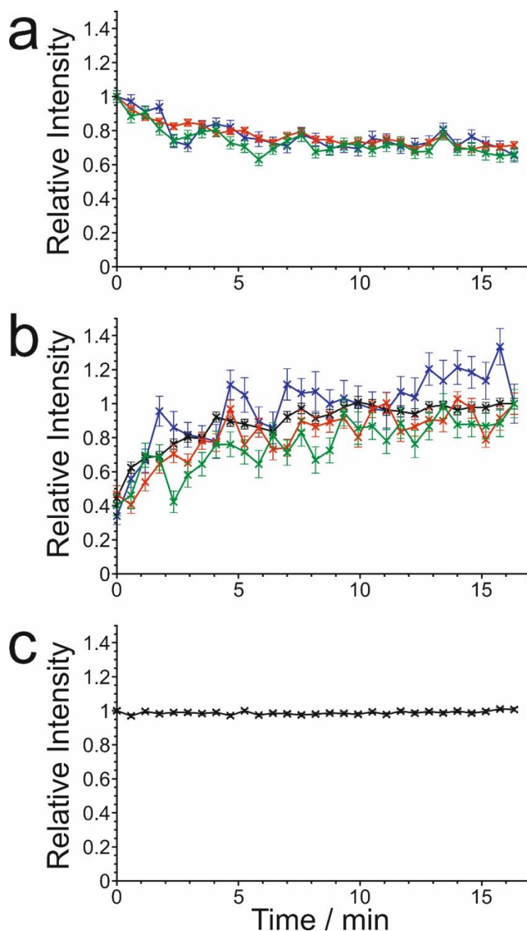
Figure 7. Relative intensities of peaks in the ^1\text{H}\rightarrow^{13}\text{C} CP NMR spectra recorded as a function of time in the CLASSIC NMR study of guest exchange for a multi-crystal sample of the 1,8-dibromooctane/urea inclusion compound in contact with liquid tetradecane, showing peaks for the three types of molecules in the urea inclusion compound: (a) 1,8-dibromooctane (the original guest), (b) tetradecane (the new guest), and (c) urea. Error bars are determined from the peak fitting process; the error bars in (c) are smaller than the symbols used to represent the data points. In (a), integrated intensities are shown for the following ^{13}\text{C} environments: \underline{\text{C}}\text{H}_2\text{Br} (blue), \underline{\text{C}}\text{H}_2\text{CH}_2\text{Br} (green), and the other ^{13}\text{C} environments at the centre of the 1,8-dibromooctane molecule combined (red). In each case, the data are scaled such that the relative intensity for the first measurement is equal to 1. In (b), integrated intensities are shown for the following ^{13}\text{C} environments: \underline{\text{C}}\text{H}_3 (blue), \underline{\text{C}}\text{H}_2\text{CH}_3 (red), \underline{\text{C}}\text{H}_2\text{CH}_2\text{CH}_3 (green), and the other ^{13}\text{C} environments at the centre of the tetradecane molecule combined (black). In each case, the data are scaled such that the relative intensity for the final measurement is equal to 1.
