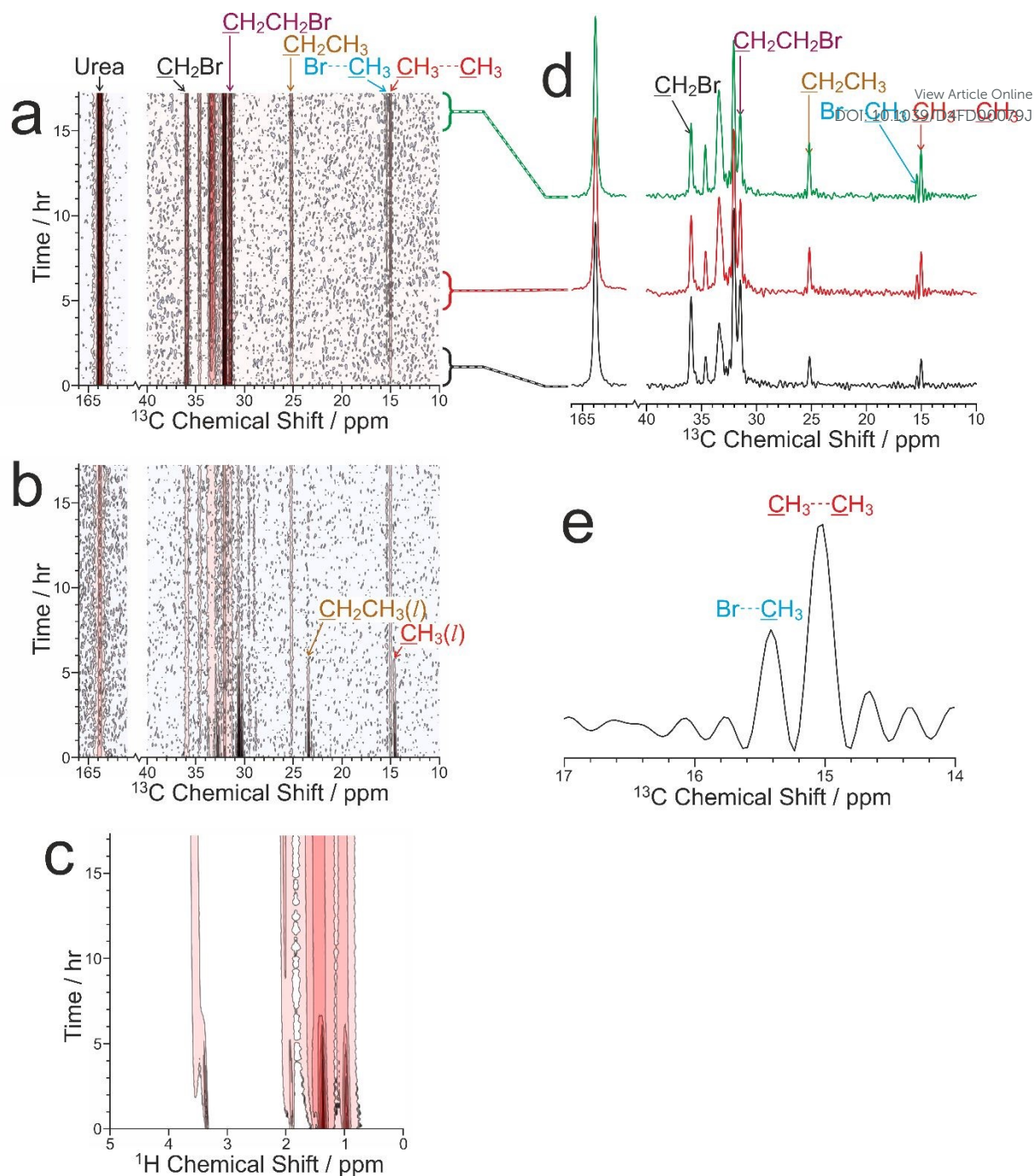
Figure 6. Intensity contour plots showing the three types of NMR spectrum recorded as a function of time during the CLASSIC NMR study of the guest exchange process for a multi-crystal sample of the 1,8-dibromooctane/urea inclusion compound in contact with liquid tetradecane: (a) ^1\text{H} \rightarrow ^{13}\text{C} CP NMR spectra, (b) direct-excitation ^{13}\text{C} NMR spectra, and (c) ^1\text{H} NMR spectra. Contours are based on a linear scale in (a) and (b) and a log scale with a factor of 2 between adjacent contours in (c). (d) ^1\text{H} \rightarrow ^{13}\text{C} CP NMR spectra recorded at different times during the guest exchange process, with the specific times indicated by the link to the time axis in (a). (e) The region of the ^1\text{H} \rightarrow ^{13}\text{C} CP NMR spectrum corresponding to the \text{CH}_3 groups of tetradecane guest molecules in the urea inclusion compound recorded at the end of the guest exchange experiment. The distorted baseline (“wiggles”) arises because the acquisition time under high-power ^1\text{H} decoupling is limited to ca. 40 ms; as a result, the end of the FID for the very sharp peaks due to the \text{CH}_3 groups is not measured.
