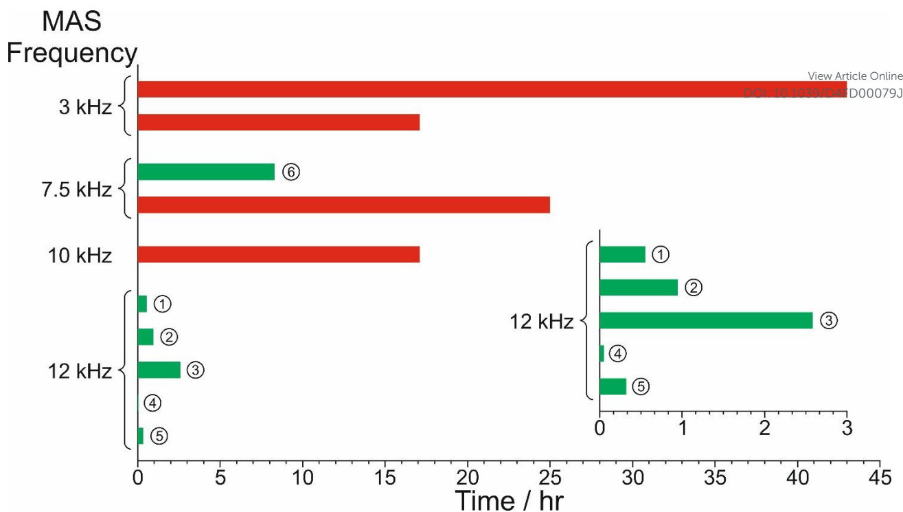
Figure 8. Summary of results from the in-situ liquid-state ^1\text{H} NMR study of crystallization of the BA-PFBA co-crystal material at different MAS frequencies. Each experiment is represented by a horizontal bar. Experiments in which crystallization was observed to occur are labelled 1 – 6, and are represented by a green bar; in each case, the length of the bar indicates the time at which the abrupt crystallization event occurred. Experiments in which crystallization was not observed are represented by a red bar; in each case, the length of the bar indicates the total time over which ^1\text{H} NMR data were measured. More information about experiments 1 – 6 is given in Table 2.
