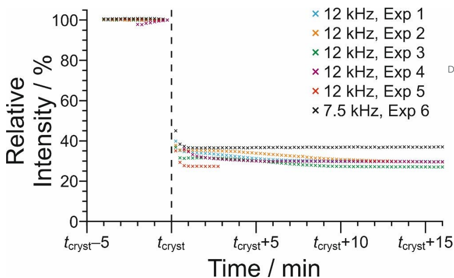
Figure 10. Variation in signal intensity as a function of time for the ^1\text{H} NMR peak due to the carboxylic acid groups of the BA and PFBA molecules in the in-situ liquid-state ^1\text{H} NMR study of crystallization of the BA-PFBA co-crystal material. The plot shows the period of time from 4 mins before the abrupt crystallization event (which occurs at time t_{\text{cryst}} ) to 16 mins after this event. Results are shown for experiments at MAS frequencies of 12 kHz (experiments 1 – 5) and 7.5 kHz (experiment 6). For each experiment, the data are normalized such that the relative peak intensity in the last spectrum recorded before t_{\text{cryst}} is 100%.
