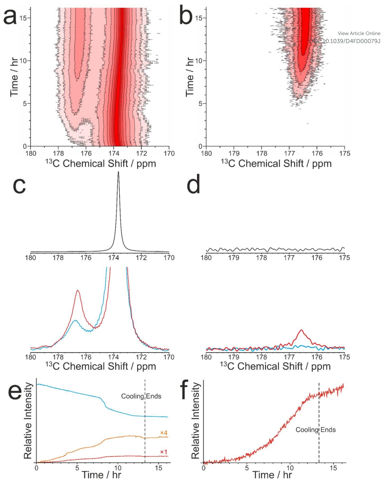
Figure 4. Intensity contour plots showing (a) the direct-excitation 13 C NMR spectra and (b) the 1 H→ 13 C CP NMR spectra recorded during the CLASSIC NMR study of crystallization of 1- 13 C-glycine from water. Contours are based on a log scale with a factor of 2 between adjacent contours. (c) Direct-excitation 13 C NMR spectra and (d) 1 H→ 13 C CP NMR spectra recorded at 0 hr (black), 4.4 hr (blue) and 8.9 hr (red). (e,f) Relative signal intensities as a function of time in the CLASSIC NMR study for (e) the direct-excitation 13 C NMR spectra and (f) the 1 H→ 13 C CP NMR spectra. In (e), the blue line represents 1- 13 C-glycine in solution, the red line represents 1- 13 C-glycine in the solid phase, and the orange line shows the same data as the red line expanded by a factor of 4.
