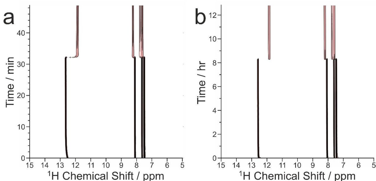
Figure 9. Intensity contour plots showing the evolution of the in-situ liquid-state ^1\text{H} NMR spectrum as a function of time during crystallization of the BA-PFBA co-crystal material at the following MAS frequencies: (a) 12 kHz (experiment 1), and (b) 7.5 kHz (experiment 6). Contours are based on a log scale with a factor of 2 between adjacent contours.
