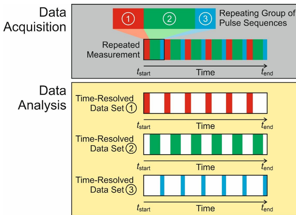
Figure 2. Schematic of the CLASSIC NMR technique, illustrated for the case in which in-situ NMR spectra are recorded as a function of time during crystallization by repeated measurement of a set of three pulse sequences (shown in red, green and blue) representing the “repeating group”. After completing the experiment, the three sets of data are separated to give a set of time-resolved NMR spectra for each of the three pulse sequences.
