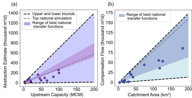
Figure 4. Relationship between (a) reservoir capacity upstream of a gauge and the reservoir abstraction volume (ABS) and (b) catchment area upstream of a gauge and compensation flow (CF). Dots represent data from a sample of catchments where abstractions could be estimated using a water balance hydrological signature and compensation flows could be extracted from drought plans, WRMPs and observed downstream flow duration curves (see Sects. 3.5.1 and S1). Dashed grey lines represent the linear transfer functions associated with the top-performing simulation from the nationally consistent calibration, the darker shading represents the spread of the top 5% of nationally consistent simulations and dashed black lines represent the limits of the transfer function parameters based on the sensitivity of model performance to these parameters (see Supplement Table S1 and Sect. S2).
