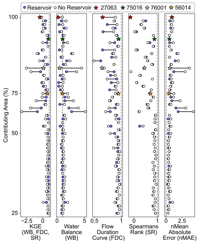
Figure 6. Difference in performance between the nationally top reservoir simulation and the nationally top no-reservoir simulation. Results are presented for the non-parametric KGE metric and its relative components as well as the normalized mean absolute error (nMAE). Catchments are ordered based on their contributing area (or proportion of the catchment that is drained through a reservoir). Dashed grey lines represent the optimum value for each metric; points falling closest to these lines have the best performance. Four catchments are highlighted using star markers and investigated in more detail in Sect. 4.4.
