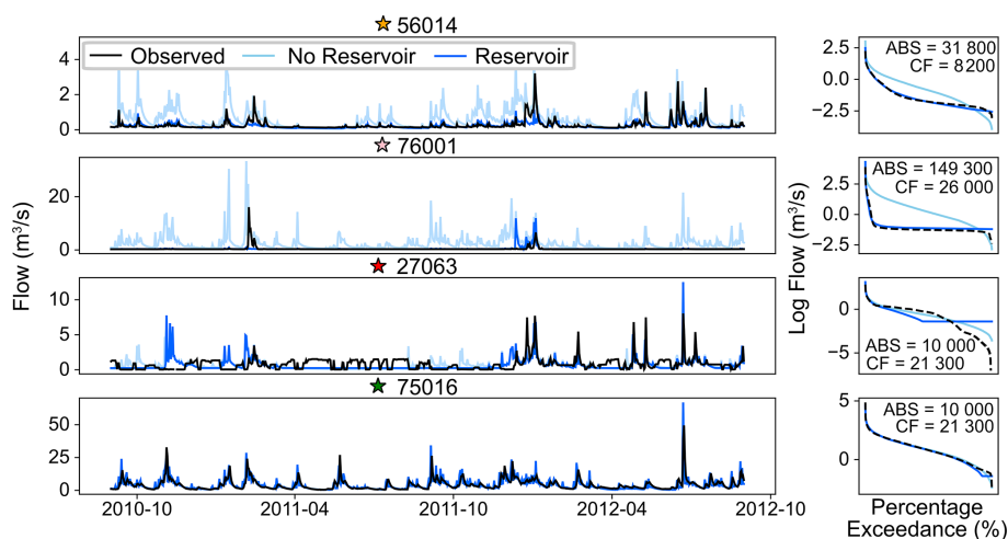
Figure 7. Hydrographs and flow duration curves from the best individual simulations (catchment-by-catchment) for selected reservoir catchments. CF and ABS are recorded on each catchment's flow duration curve in \text{m}^3 \text{d}^{-1} .
