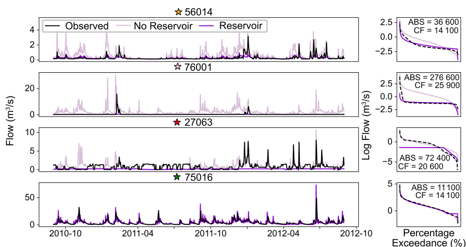
Figure 8. Hydrographs and flow duration curves from the best median simulation (nationally consistent calibration) for selected reservoir catchments. CF and ABS are recorded on each catchment's flow duration curve in \text{m}^3 \text{d}^{-1} .
