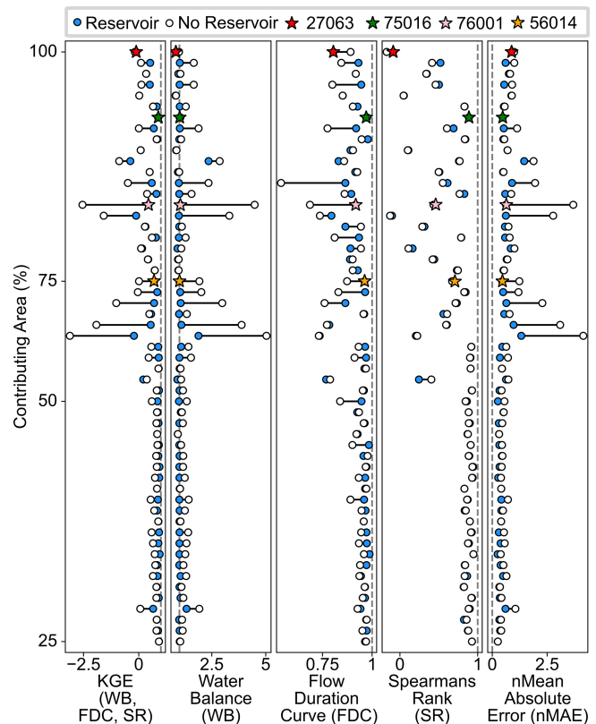
Figure 5. Difference in performance between the top reservoir simulation in each catchment and the top no-reservoir simulation. Results are presented for the non-parametric KGE metric and its relative components as well as the normalized mean absolute error (nMAE). Catchments are ordered based on their contributing area (proportion of the catchment that is drained through a reservoir). Dashed grey lines represent the optimum value for each metric; points falling closest to these lines have the best performance. Four catchments are highlighted using star markers and investigated in more detail in Sect. 4.4.
