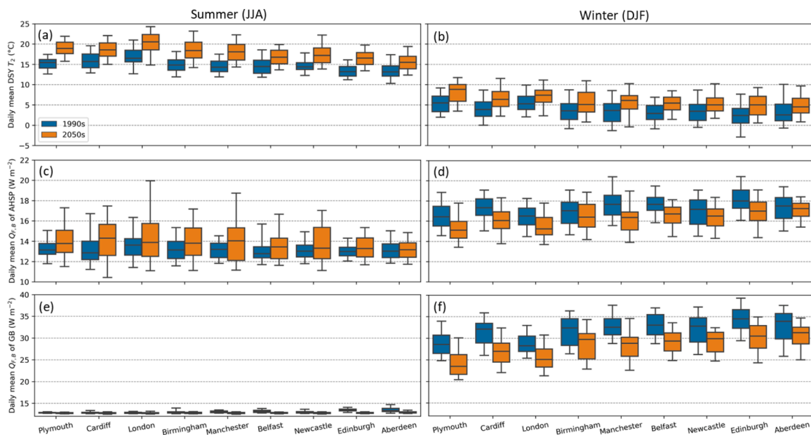
Fig. 12. For flats in UK cities (with increasing latitude, Fig. 4c) under 1990s and 2050s (colour) for (a, c, e) summer (JJA) and (b, d, f) winter (DJF) climate, the variability of the daily mean (a, b) 2 m DSY air temperature ( T_2 ) (monthly values shown in Fig. 4a, b), (c, d) anthropogenic heat emissions ( Q_{F,B} ) from ASHP, and (e, f) Q_{F,B} from gas boilers. Median (horizontal line), interquartile range (box), and 5 th and 95 th percentiles (whiskers) shown. London 2050s Q_{F,B} results given in Fig. 5b.
