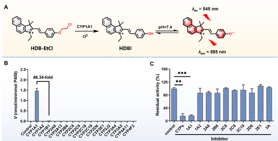
Figure 2 (A) Sensing mechanism of HDB-EtCl towards hCYP1A1. (B) HDB-EtCl was incubated with each tested human CYP enzyme for 30 min under physiological conditions (37 °C, pH 7.4). (C) The inhibitory effects of CYP inhibitors on HDB-EtCl O -dechloroethylation in human liver preparations. Data are presented as mean \pm SD ( n = 3 ). ** P < 0.01 , and *** P < 0.001 .
