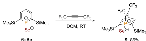
Scheme 3. [4+2] Cycloaddition of F_3CC\equiv CCF_3 to phosphinine selenide 6=Se .
