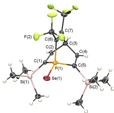
Figure 5. Molecular structure of 9 in the crystal. Displacement ellipsoids are shown at the 50% probability level. Selected bond lengths (Å) and angles (°): P(1)–Se(1): 2.0880(8); P(1)–C(1): 1.816(3); P(1)–C(5): 1.821(3); C(1)–C(2): 1.320(4); C(2)–C(3): 1.536(4); C(3)–C(4): 1.533(4); C(4)–C(5): 1.320(4); C(3)–C(7): 1.526(4); P(1)–C(6): 1.857(3); \Sigma \angle (C–P–C) 296.10(14).
