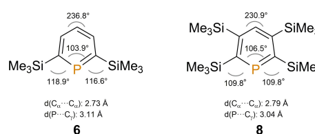
Figure 6. Calculated bond angles and distances in 6 and 8 .
