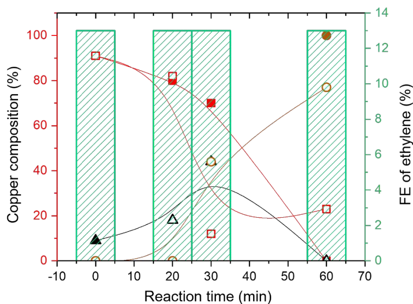
Fig. 7. A correlation between the copper composition (Tables 1 and 2) and FE of ethylene (Fig. 3) as a function of reaction time. The open and filled symbols reflect the bulk composition derived from in situ XANES and surface composition deduced from quasi in situ XPS, respectively. Copper composition: Cu(II) (■;□), Cu(I) (▲;Δ) and Cu 0 (●;○).
