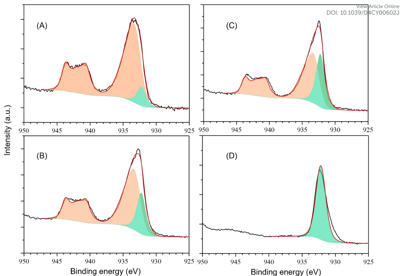
Fig. 6. High resolution quasi in situ XPS spectra, including peak fitting, of Cu 2p of Cu-GDE during the reaction: the Cu-GDE at time 0 (A), 20 (B), 30 (C) and 60 (D) min. Refer to experimental sections (2.3 and 2.7) for details. The sum of the components of each oxidation state is presented for clarity.
