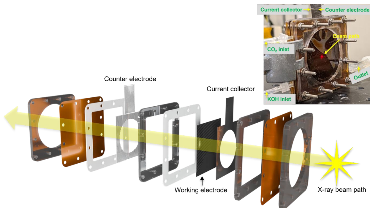
Fig. 1. CAD image of the operando XAS – GDE flow cell. The inset photograph shows the cell setup on the beamline.
