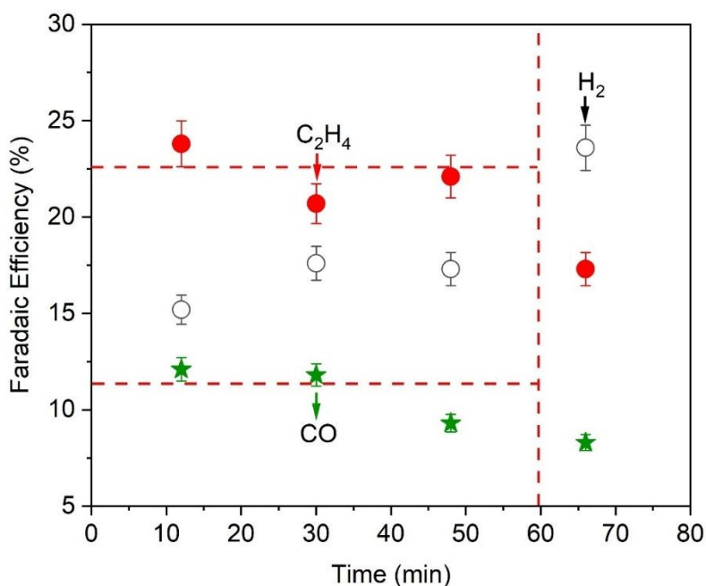
Fig. 3. eCO 2 R over operando XAS-Cu-GDE flow cell: the FE (%) of gaseous products are plotted as a function of time. Vertical and horizontal dashed lines are included for guidance purposes. Refer to experimental section 2.4 for details.
