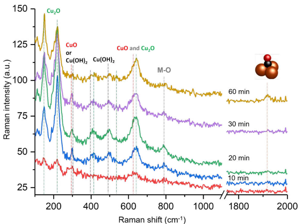
Fig. 5. Quasi in situ Raman spectra collected during the eCO 2 R reaction. General peak assignment is indicated by the dashed lines. M – O indicates copper-oxygen bond. Bridge bound CO adsorption on metallic Cu at 1920 cm -1 is depicted. Refer to experimental sections 2.3 and 2.6 for details.
