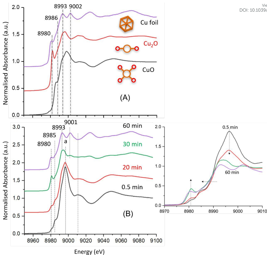
Fig. 4. XANES spectra of reference copper samples (A) and in situ XANES spectra of Cu-GDE during the eCO 2 R reaction (B). 'a' in the panel (B) indicates the white line of the XANES spectra collected within 20 min and inset of the panel (B) shows the overlaid and magnified region of the in situ XANES spectra for better visibility of the changes. Refer to experimental sections 2.4 and 2.5 for details. The vertical dashed lines in panels (A) and (B) indicate the energies of the pre-edge features, edge position and edge features. Arrows in the inset of the panel (B) indicate the change in intensities of the features and edge position.
