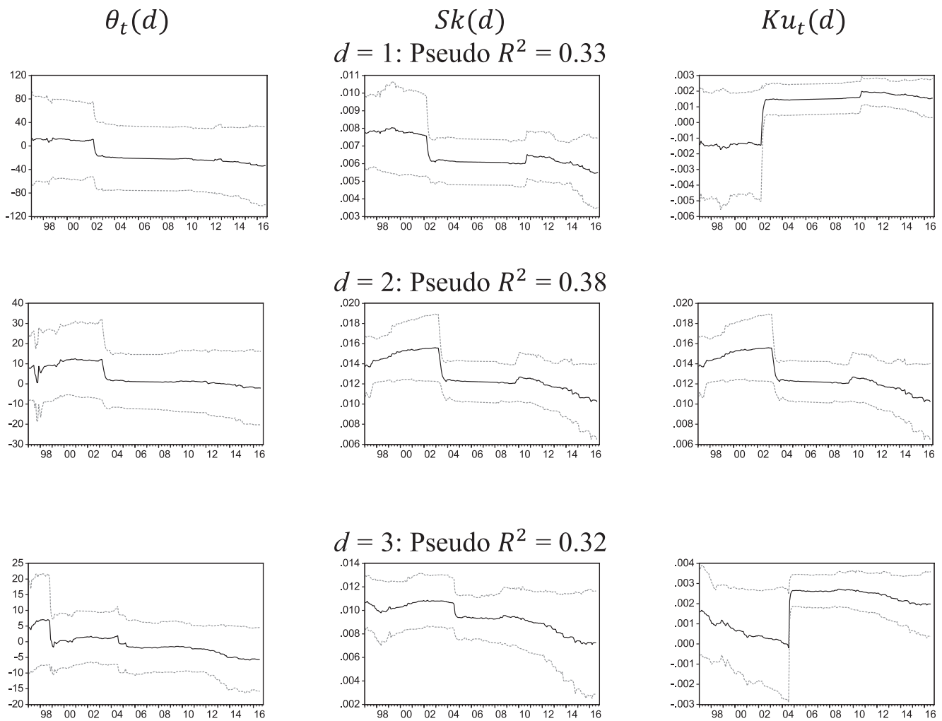
FIGURE 3 | Estimated time-varying coefficients: EU – CPI \theta_t(d) .
