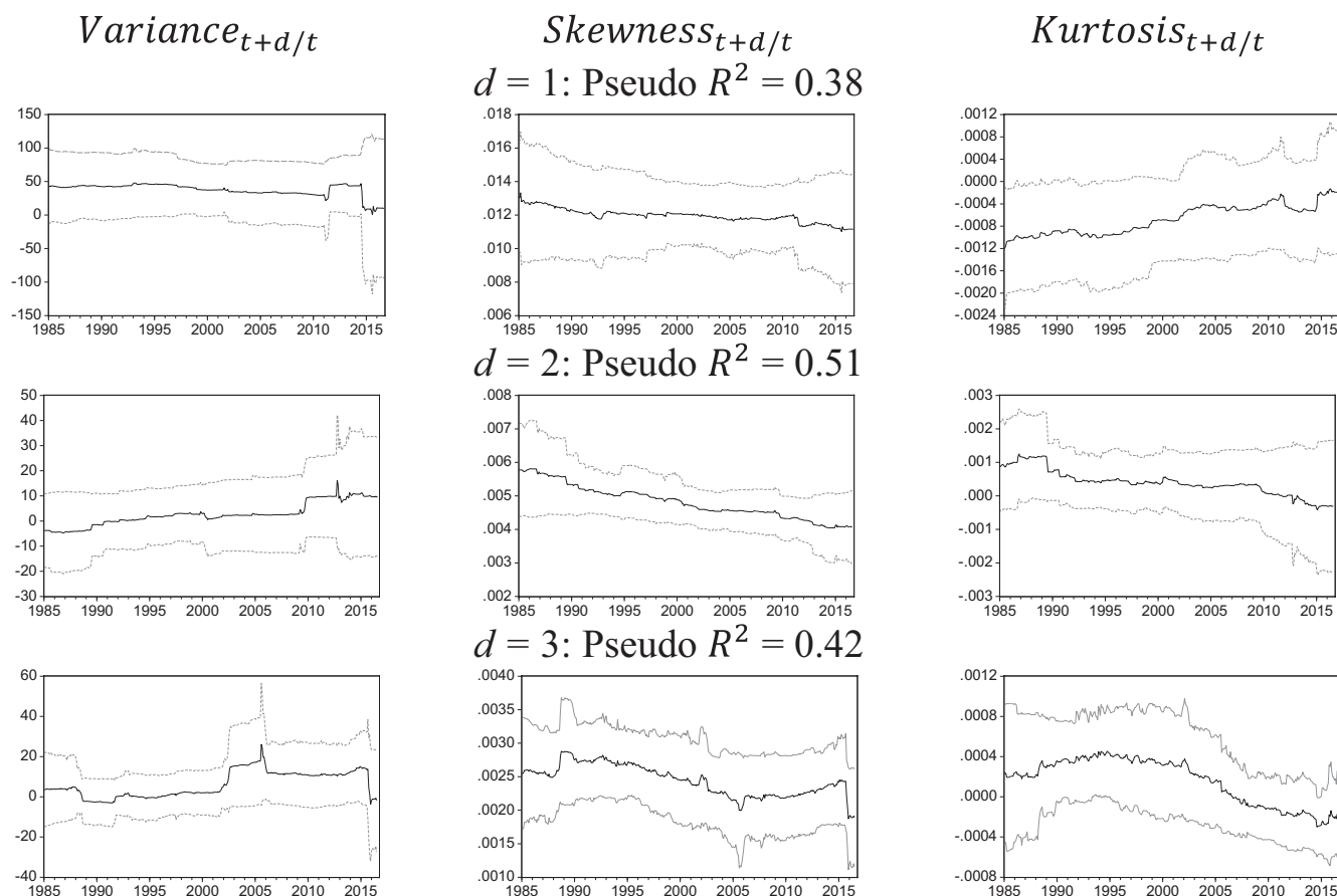
FIGURE A3 | Estimated time-varying coefficients: Japan – PPI.
