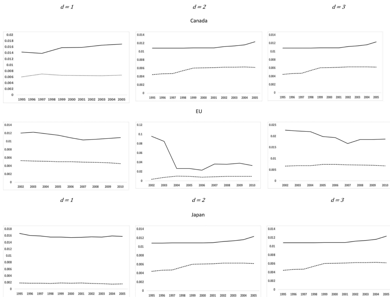
FIGURE 5 | Percentiles of confidence intervals of skewness coefficients from rolling samples*. *The focus period is set to January 1995 through December 2005 for CA/USA and JP/USA, and from January 2002 to December 2010 for EU/USA. The rolling samples for CA/USA and JP/USA are fixed to 252 observations, starting from January 1, 1985, and rolling over for one year until and including January 1, 1994. For EU/USA, the rolling sample is fixed to 168 observations, starting from January 1, 1997, and rolling over for 1 year until and including January 1, 2002. The percentiles reported in the figures are the 97.5th for the upper bound of the confidence interval and the 2.5th for the lower bound. The real exchange rates are computed using CPI.
