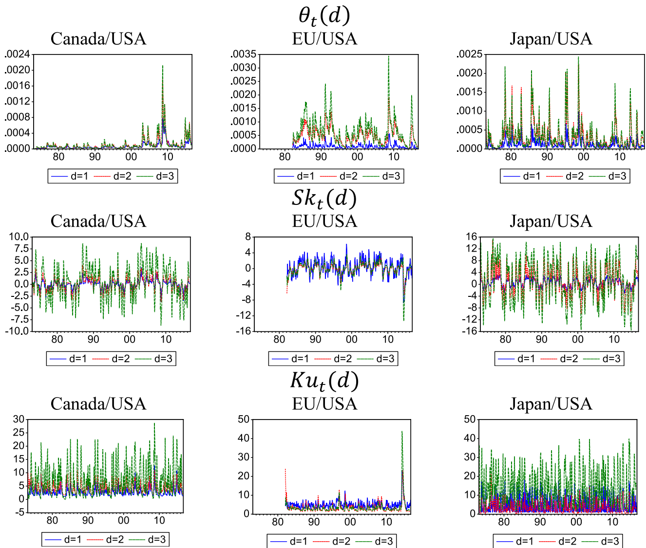
FIGURE 1 | Estimated higher moments of bilateral exchange rate. [Colour figure can be viewed at wileyonlinelibrary.com ]
