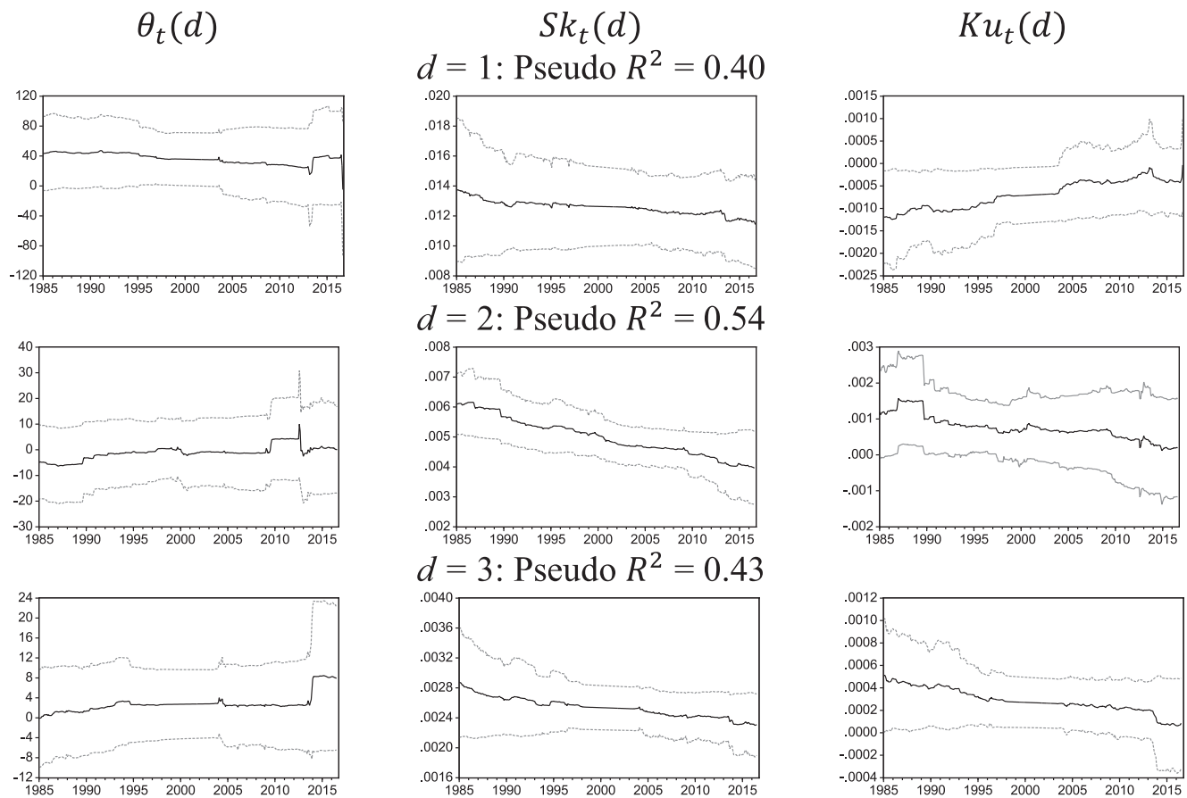
FIGURE 4 | Estimated time-varying coefficients: Japan – CPI.
