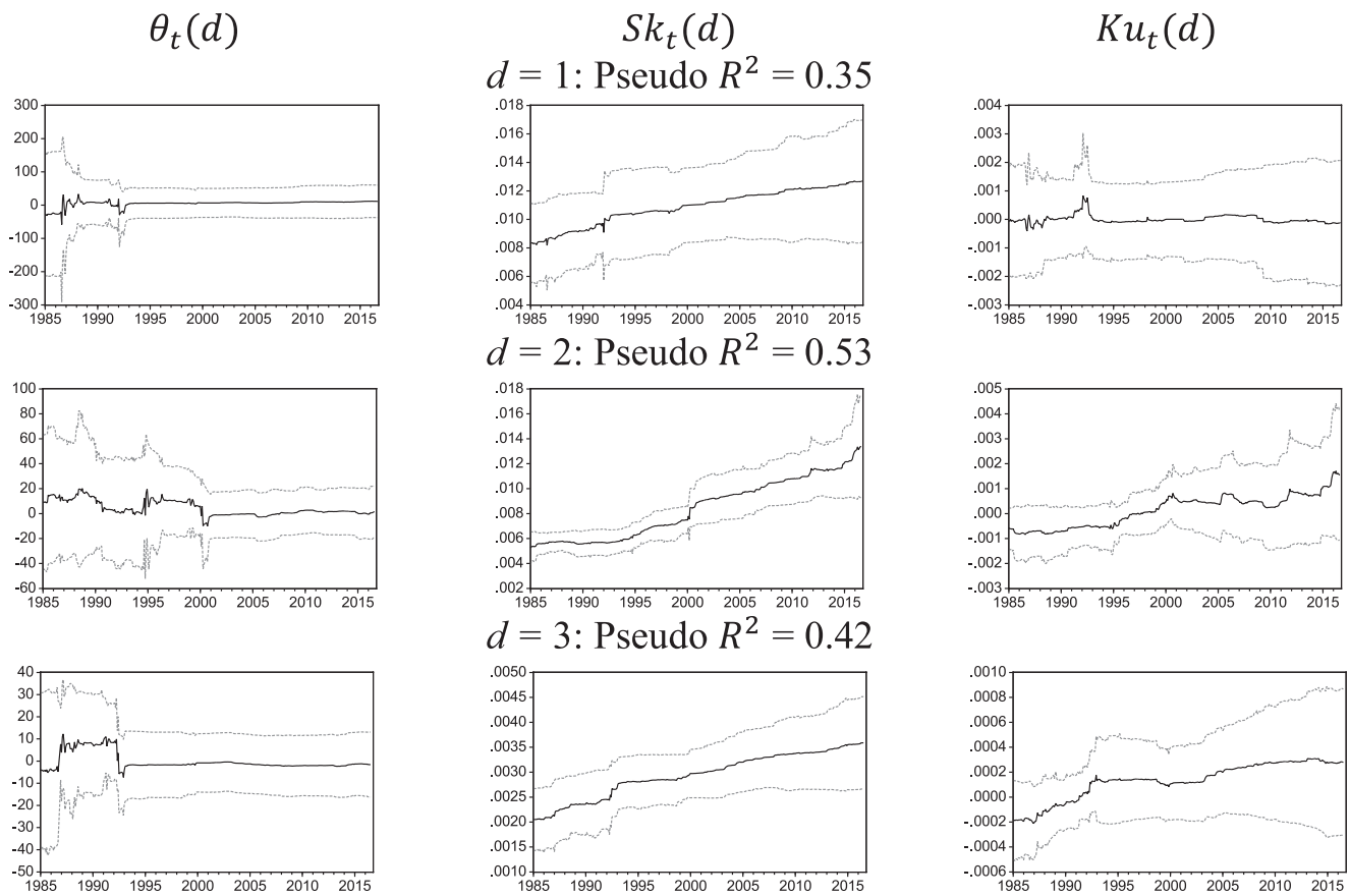
FIGURE 2 | Estimated time-varying coefficients: Canada – CPI.
