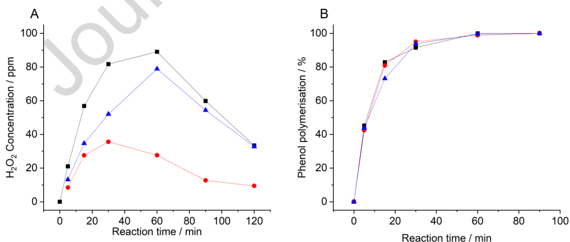
Figure 2. The effect of reaction solution pH on (A) the direct synthesis of \text{H}_2\text{O}_2 and (B) the chemo-enzymatic polymerisation of phenol, as a function of pH. Key for Figure 2: pH 6 (black squares), pH 7 (red circles) and pH 8 (blue triangles). \text{H}_2\text{O}_2 direct synthesis reaction conditions: Catalyst (0.001 g), phosphate buffer (100 mM, 10 mL), using a gas mixture of 80% \text{H}_2 /air (23 psi \text{H}_2 , 6 psi air), 20 °C, 250 rpm. Chemo-enzymatic phenol polymerisation reaction conditions: chemo-catalyst (0.001 g), HRP
