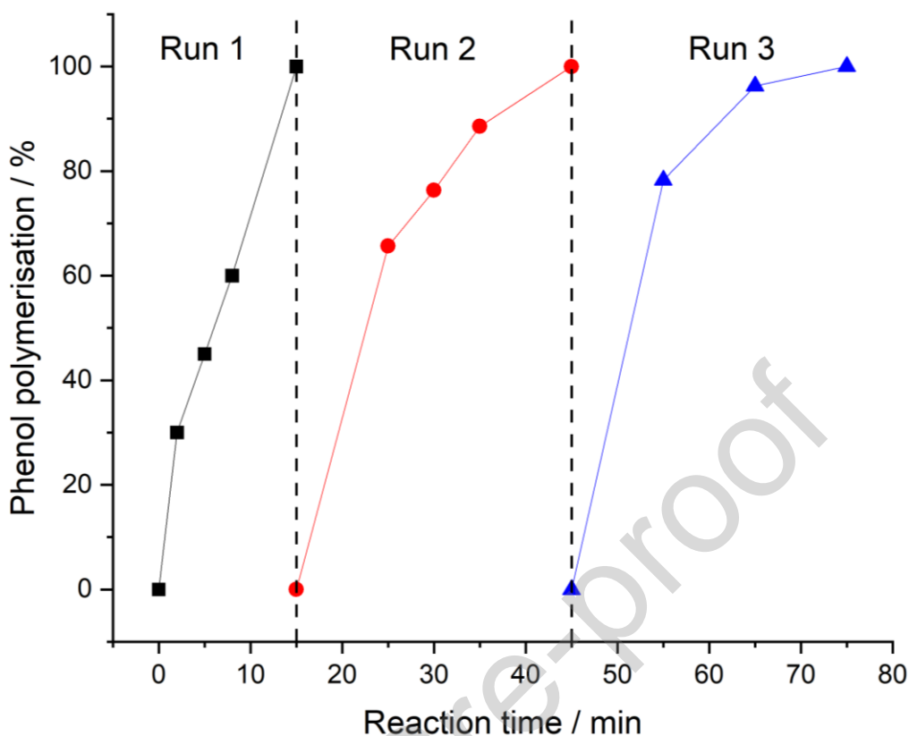
Figure 5. Stability of the chemo-enzymatic system, over successive phenol polymerisation reactions. Key: dashed lines indicate substrate (phenol, H 2 and O 2 ) recharging. Chemo-enzymatic phenol polymerisation reaction conditions: catalyst (0.001 g), HRP (4U mL -1 ) phenol (0.3 mM), phosphate buffer (50 mM, 10 mL, pH 8.0), using a gas mixture of 80 % H 2 /air (23 psi H 2 , 6 psi air), 20 °C, 250 rpm.
