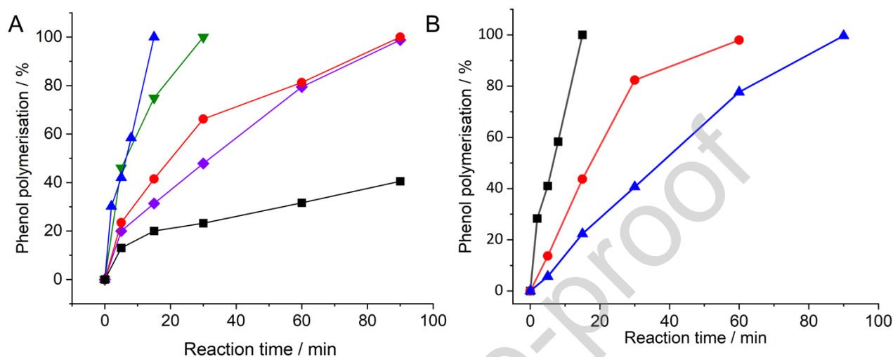
Figure 1.A. The catalytic activity of 1%AuPd/TiO 2 catalysts, when used in conjunction with HRP, towards the conversion of phenol. Key for Figure 1.A: 1%Au/TiO 2 (black squares), 0.75%Au-0.25%Pd/TiO 2 (red circles), 0.5%Au-0.5%Pd/TiO 2 (blue triangles), 0.25%Au-0.75%Pd/TiO 2 (inverted green triangles) and 1%Pd/TiO 2 (purple diamonds). B. The performance of the 0.5%Au-0.5%Pd/TiO 2 /HRP chemo-enzymatic system towards phenol polymerisation, as a function of phenol concentration. Key for Figure 1.B: 0.3 mM phenol (black squares), 0.6 mM phenol (red circles), 1.2 mM phenol (blue triangles). Chemo-enzymatic phenol polymerisation reaction conditions: chemo-catalyst (0.001 g), HRP (4 U mL -1 ) phenol (0.3 -1.2 mM), phosphate buffer (50 mM, 10 mL, pH 8.0), using a gas mixture of 80 % H 2 /air (23 psi H 2 , 6 psi air), 20 °C, 250 rpm.
