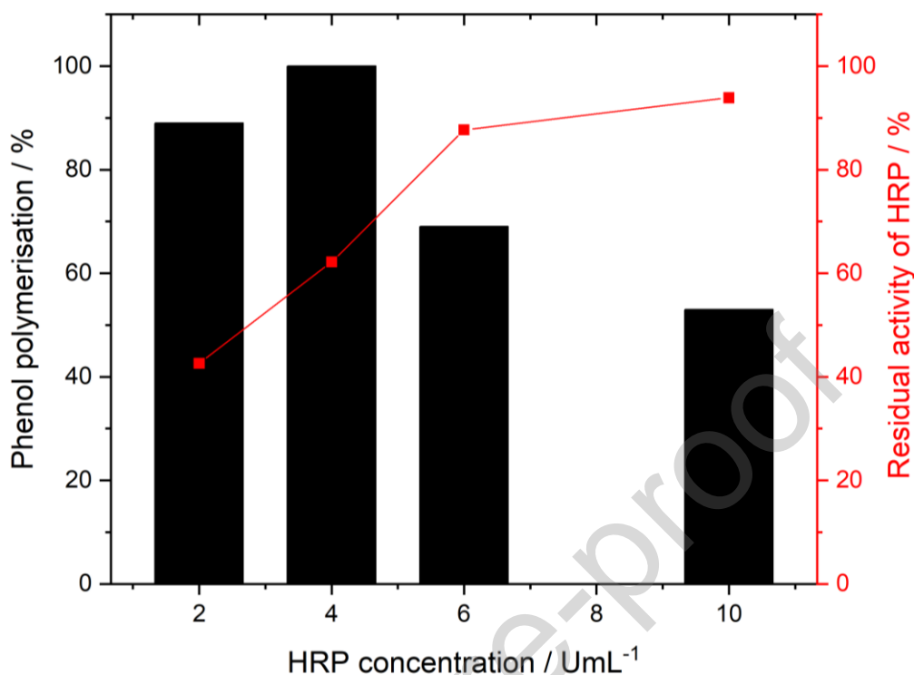
Figure 4. The effect of HRP concentration on chemo-enzymatic polymerisation of phenol. Reaction conditions: chemo-catalyst (0.001 g), HRP (2-10 U mL -1 ) phenol (0.3 mM), phosphate buffer (50 mM, 10 mL, pH 8.0), using a gas mixture of 80 % H 2 /air (23 psi H 2 , 6 psi air), 20 °C, 250 rpm, 15 min.
