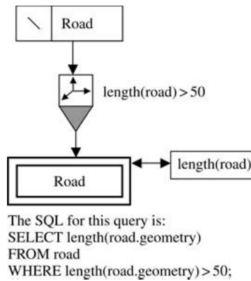
Figure 34. A spatial filter in a simple query.
