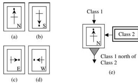
Figure 20. Directional spatial joins.
