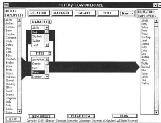
Figure 2. Graphical filter flow [53].
