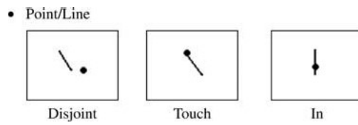
Figure 14. Point/line spatial relationships.
