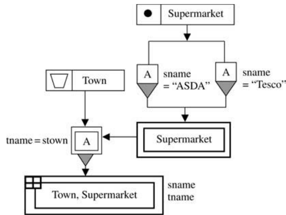
Figure 36. Example query of a non-spatial join.
