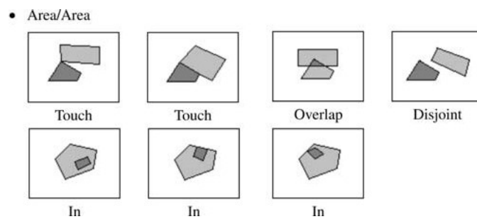
Figure 16. Area/area spatial relationships.
