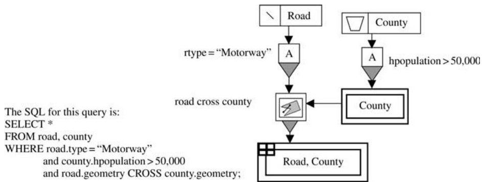
Figure 37. Example query of a spatial join. Specific relationship icon replaces general spatial join to indicate the cross relationship.
