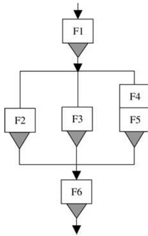
Figure 32. Filter configuration: (F1 AND (F2 OR F3 OR (F4 AND F5)) AND F6).
