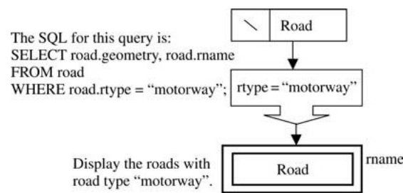
Figure 6. Result box in query.
