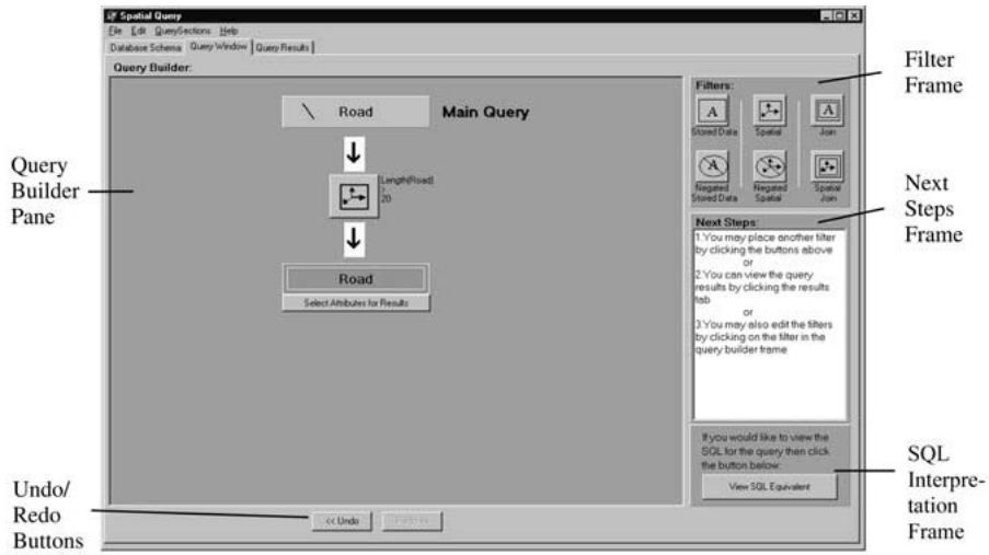
Figure 39. Query formulation page.
