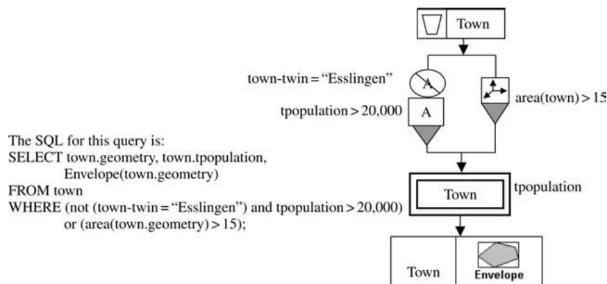
Figure 35. A query that uses and, or and not.
