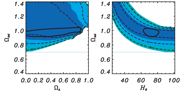
Fig. 3. Likelihood contours in the (\Omega_A, \Omega_{\text{tot}}) (left) and (H_0, \Omega_{\text{tot}}) (right) planes using the Archeops dataset; the three colored regions (three contour lines) correspond to resp. 68, 95 and 99% confidence levels for 2-parameters (1-parameter) estimates. Black solid line is given by the combination Archeops + HST, see text.
