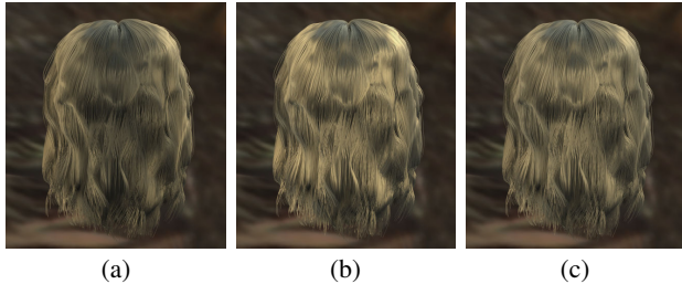
Figure 9: Editing index of refraction \eta and the azimuthal width w_c for the TRT caustic. (a) \eta = 1.54 , w_c = 0.06 ; (b) \eta = 1.65 , w_c = 0.06 ; (c) \eta = 1.65 , w_c = 0.20 .
