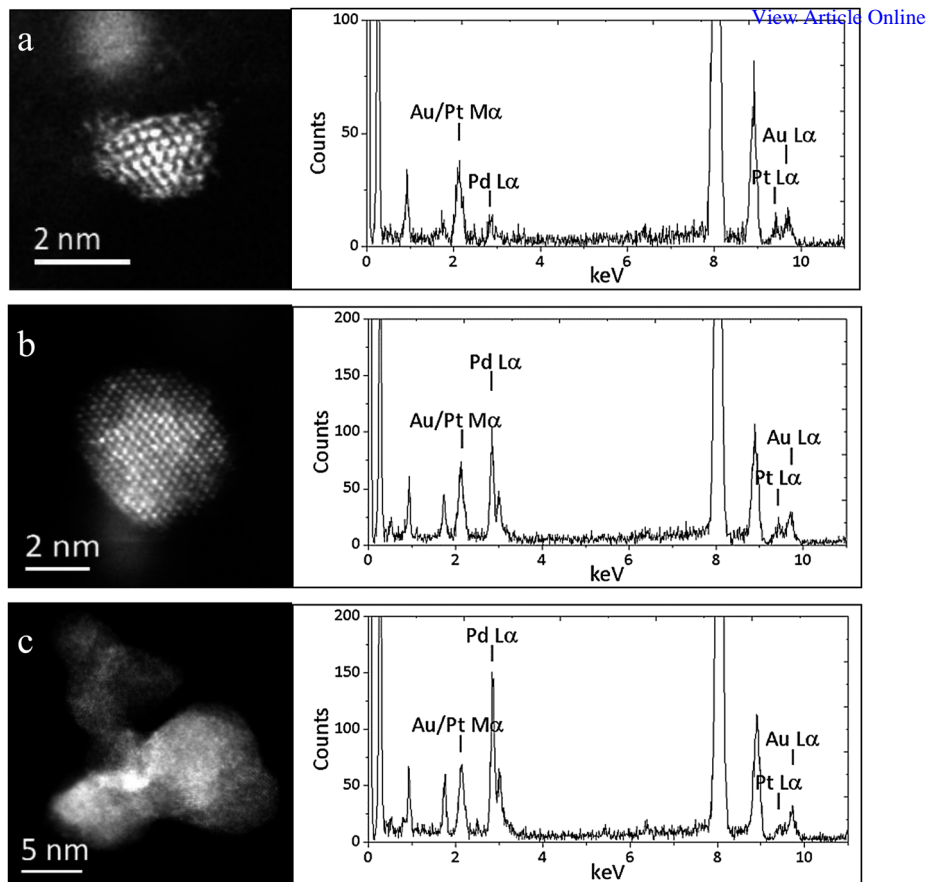
Fig. 4 Representative high magnification STEM-HAADF images and the corresponding X-ray energy dispersive spectra acquired from representative (a) 2 nm, (b) 5 nm and (c) 10 nm particles in the sol-immobilized 1 wt% (0.3Au + 0.4Pd + 0.3Pt)/C trimetallic catalyst dried at 120 °C.
