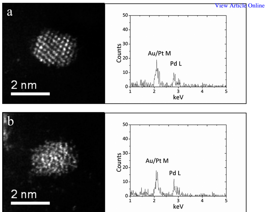
Fig. 8 (a) An HAADF image and the corresponding XEDS spectra from a 2 nm Au–Pd–Pt particle in a 1 wt% (0.3Au + 0.4Pd + 0.3Pt)/C trimetallic catalyst prepared by the sol-immobilization method; (b) A second consecutive HAADF image and corresponding XEDS spectra of the same particle. A comparison of these two datasets indicates that the composition quantification from XEDS spectra was not significantly affected by electron beam damage under the experimental conditions employed.
