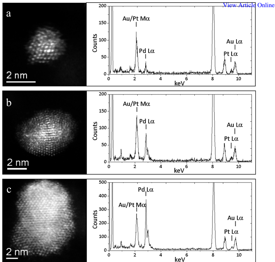
Fig. 3 High magnification STEM-HAADF images and the corresponding X-ray energy dispersive spectra acquired from representative (a) 2 nm, (b) 5 nm and (c) 10 nm particles in the sol-immobilized 1 wt% (0.45Au + 0.45Pd + 0.1Pt)/C catalyst dried at 120 °C.
