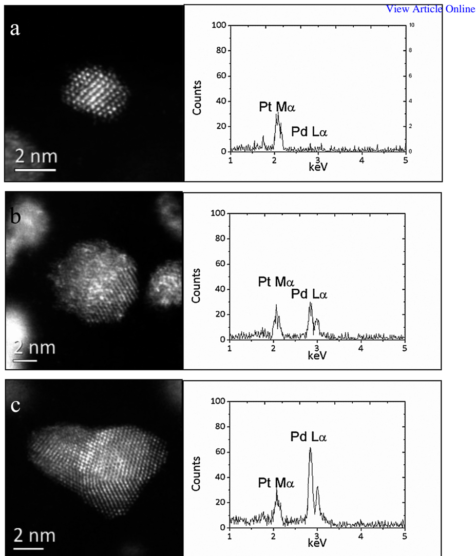
Fig. 5 Representative high magnification STEM-HAADF images and the corresponding X-ray energy dispersive spectra acquired from representative (a) 2 nm, (b) 5 nm and (c) 10 nm particles in the sol-immobilized 1 wt% (0.5Pd + 0.5Pt)/C bimetallic catalyst dried at 120 °C.
