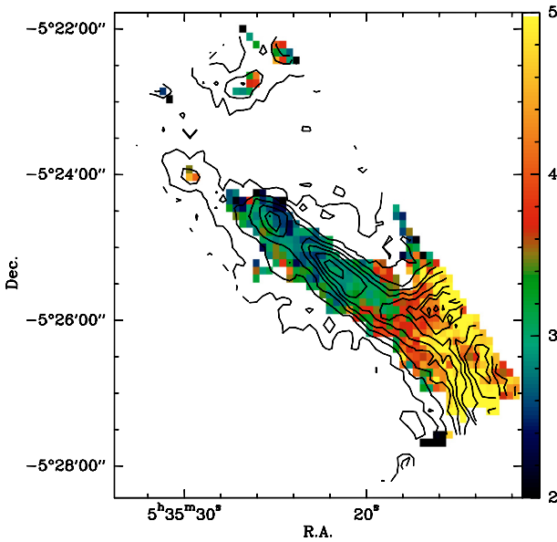
Fig. 9. Ratio of the integrated intensity of the \text{H}_2\text{CO} 3_{0,3}-2_{0,2} transition to the 3_{2,2}-2_{2,1} . The solid black contours show the integrated intensity of the 3_{0,3}-2_{0,2} line (levels are from 1.8 \text{K km s}^{-1} in steps of 1.8). Typical errors along the Bar are of the order of 0.3.
