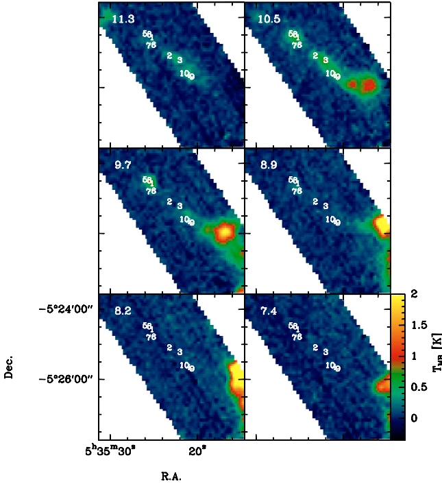
Fig. 7. Channel maps of the CH 3 OH-A ( 5_0-4_0 ) emission between 11.3 and 7.4 km s -1 observed with the IRAM-30 m telescope.
