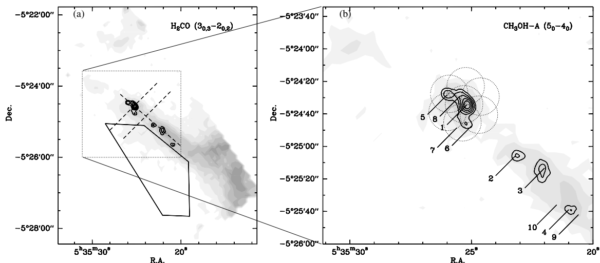
Fig. 1. In grey scale, the integrated intensity of the \text{H}_2\text{CO} ( 3_{0,3}-2_{0,2} ) line ( left ) and of the \text{CH}_3\text{OH-A} ( 5_0-4_0 ) transition ( right ) observed with the IRAM-30 m telescope. Black contours (4, 8, and 12 times 0.032 \text{ Jy beam}^{-1} \text{ km s}^{-1} ) show the distribution of the \text{H}^{13}\text{CN} ( 1-0 ) emission observed with the Plateau de Bure interferometer (Lis & Schilke 2003). For \text{H}_2\text{CO} the contours start from 1.8 \text{ K km s}^{-1} in steps of 1.8 (equal to 3\sigma ), for \text{CH}_3\text{OH} from 0.3 \text{ K km s}^{-1} in steps of 0.3 (equal to 3\sigma ). In the left panel , the dashed lines indicate the strips used for Fig. 6; the solid lines outline the regions used to derive the average \text{H}_2\text{CO} and \text{CH}_3\text{OH} emission in the interclump material (Figs. 3b and 4c); the dotted lines mark the region shown in the right panel . In the right panel , the numbers label the positions of the clumps detected in \text{H}^{13}\text{CN} ; the dotted circles outline the mosaic of seven fields observed with the PdBI (see Sect. 2.2).
