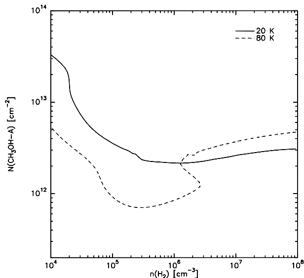
Fig. 11. Results of the statistical equilibrium calculations for CH 3 OH. The solid and dashed lines show the line intensity of the 5 0 –4 0 -A line as measured towards the interclump medium (0.06 K) for temperatures of 20 and 80 K, respectively, as functions of density and column density of CH 3 OH-A.
