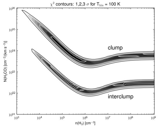
Fig. 10. \chi^2 square distribution of the 3_{0,3}-2_{0,2} and 3_{2,2}-2_{2,1} line intensities in the [n(\text{H}_2), N(\text{H}_2\text{CO})] plane for a temperature of 100 K for the two sets of observations clump and interclump shown in Fig. 3. The plot shows, for each spatial region, the low-density branch and the high-density branch discussed in the text. Note that to derive the column densities given in Sect. 4.1, one has to multiply with the line widths.
