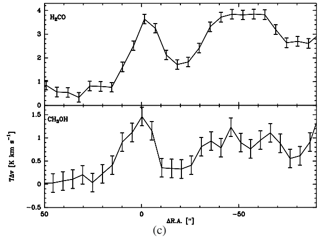
Fig. 6. Variation in the integrated intensity of the CH 3 OH-A (5 0 –4 0 ) and H 2 CO 3 2,2 –2 2,1 lines observed with the IRAM-30 m telescope across clumps 1 (a), the interclump medium between clump 1 and 2 (b) and along the Bar (c). In Fig. 1 we outline the strips used to extract the plots.
