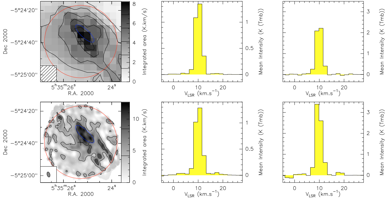
Fig. 8. Top line: IRAM-30 m data. Bottom line: hybrid 30 m+PdBI deconvolved data cube. Left column: images of the integrated line intensity of the \text{H}_2\text{CO} ( 3_{0,3}-2_{0,2} ) transition between 8.3 and 11.7 \text{km s}^{-1} . The values of the contour levels are shown on the colour scale. Middle column: spectra averaged over the whole interferometric field-of-view marked as the red circle on the images. Right column: spectra averaged over the central clump marked with the blue ellipse on the images.
