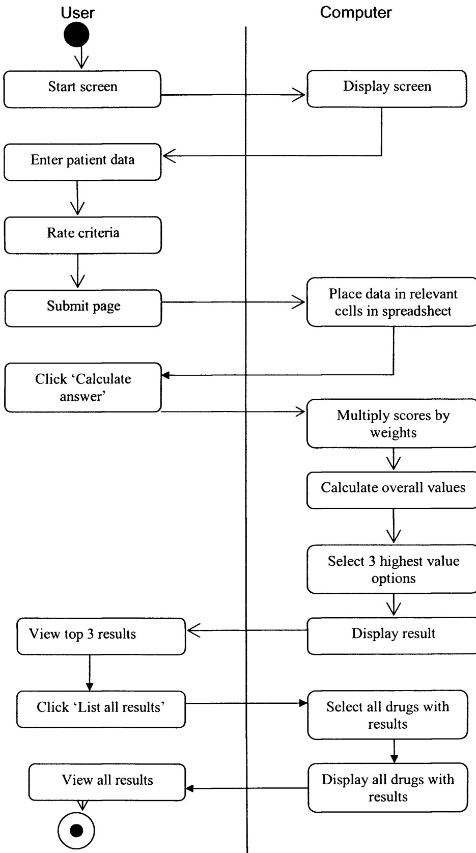
Figure 5.7 Activity diagram
