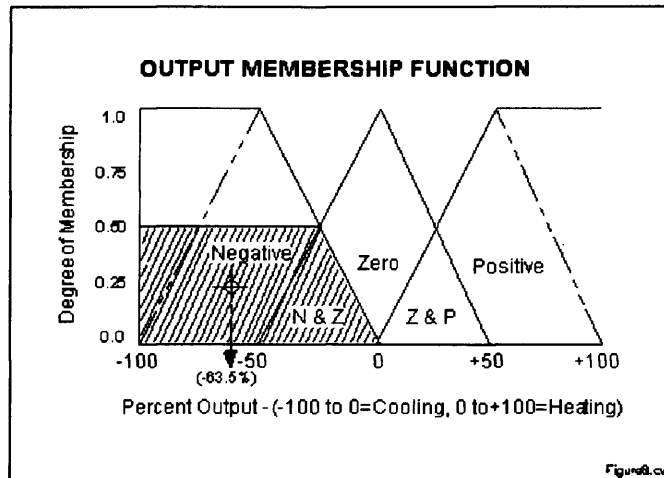
Fig. 4.4 - The horizontal coordinate of the centroid is taken as the crisp output
