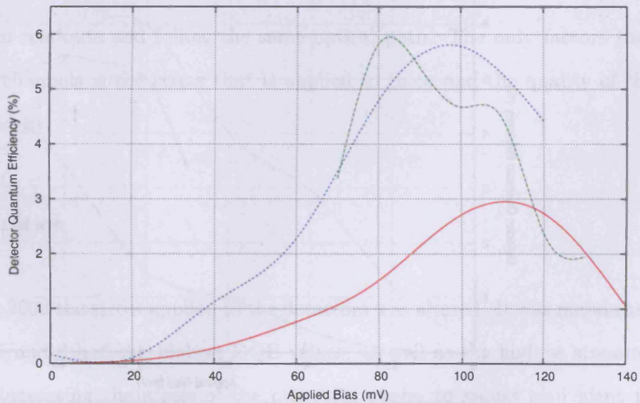
Figure 3.2: Comparison of detector quantum efficiency (%) varying with applied bias (mV) for channels three and four. Data were taken during three separate periods with a cold plate of 3.7 K for all.
