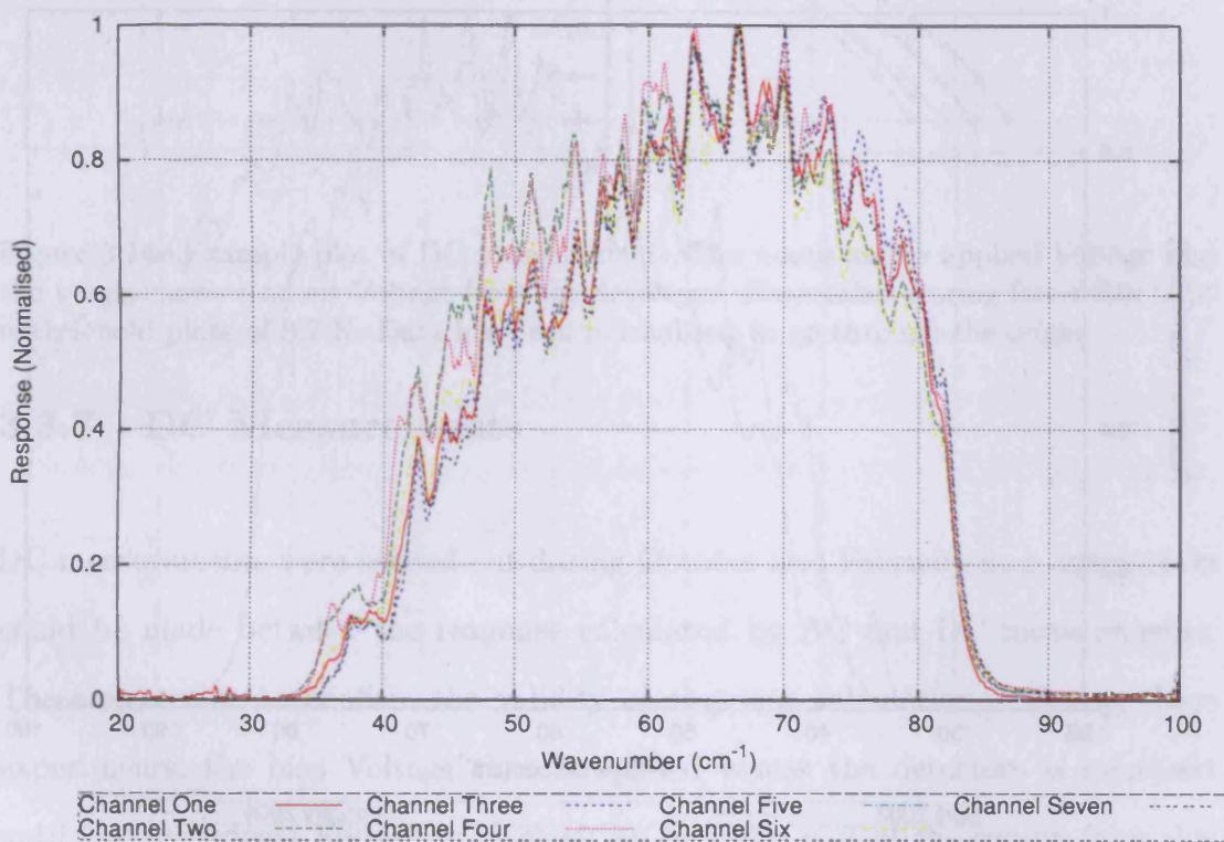
Figure 3.12: Spectral response measurement for all THUMPER's detectors. Data taken during June 2004 with a cold plate of 4.2 K and 90 cm^{-1} low pass edge filters on the cryogenic shields only. Each channel has been normalised against itself.
