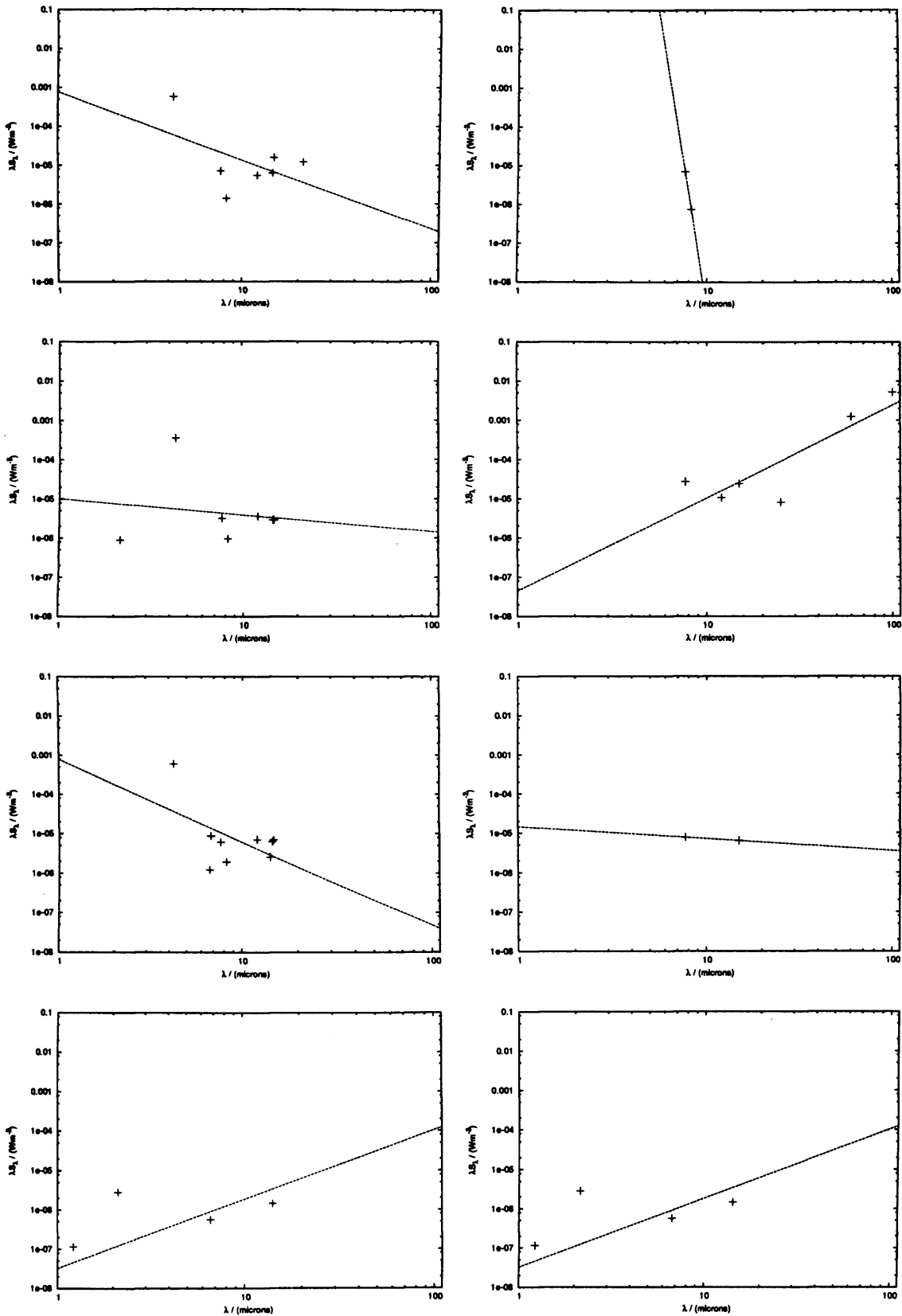
Figure 6.5: SEDs for IR sources associated with methanol masers 33 (bottom left) to 40 (top right)
