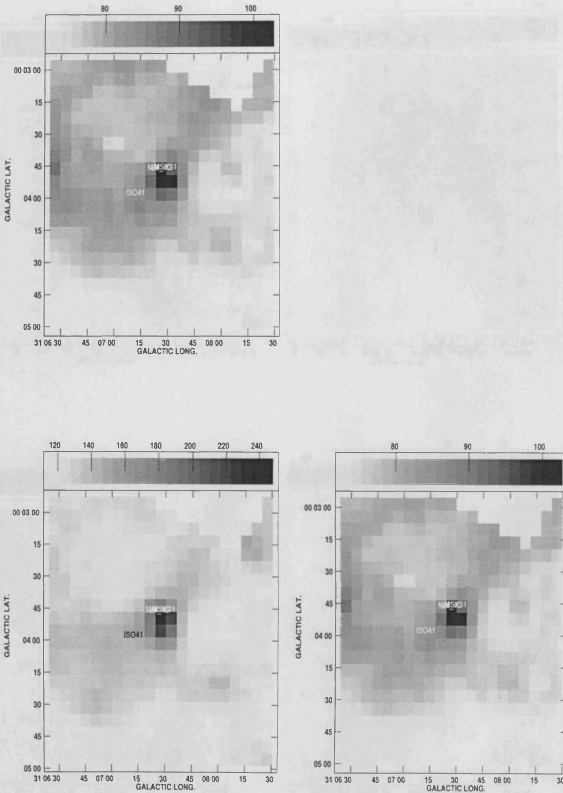
Figure 5.20: ISO images associated with methanol maser 40
