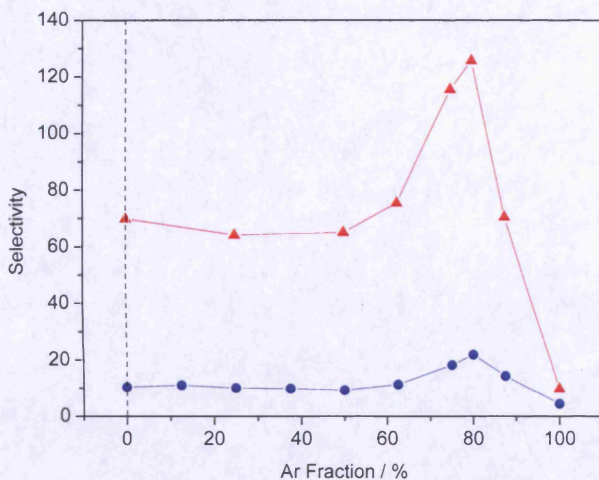
Figure 5.19 - Selectivity of the AlGaInP etch with respect to SiO 2 (blue circles), and Ni (red triangles) masks as a function of Ar fraction at 190°C (all other conditions as in Table 5.1, dashed vertical line shows the 'standard' conditions).
