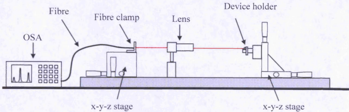
Figure 6.6 – Experimental setup for measuring laser wavelength.
