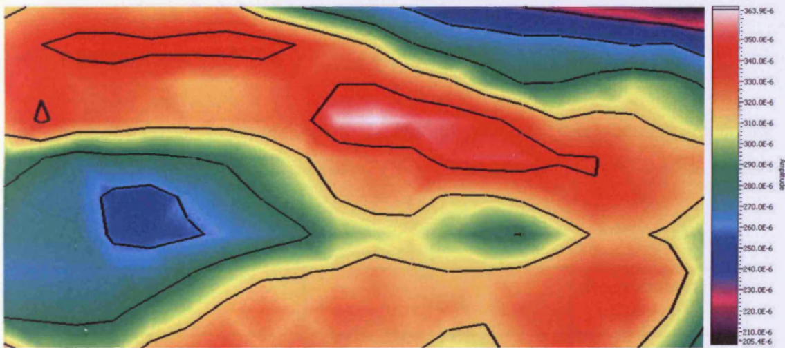
Figure 5.4. Typical image of rms Barkhausen noise scanned over, 40 mm × 20 mm, with a step size of 1 mm, on a grain-oriented electrical steel sample at magnetising frequency of 50 Hz and peak flux density of 1 T
