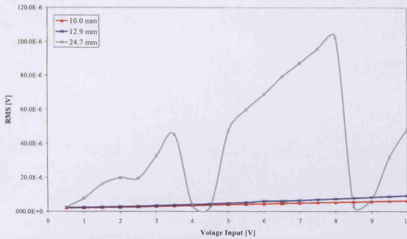
Figure 4.46. Non-magnetic sample test for ferrite length investigation
