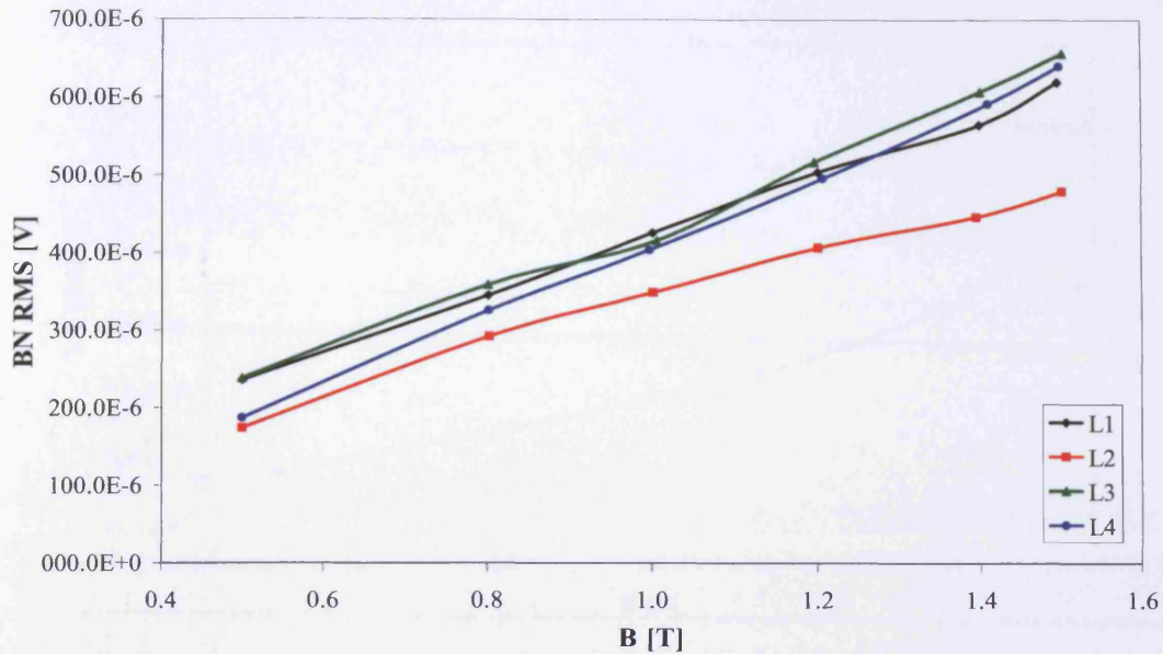
Figure 6.39. Variation of rms Barkhausen noise, BN RMS, with peak magnetic flux density, B , at 50 Hz magnetising frequency, for uncoated 3%Si sample, measured with the ferrite sensor
