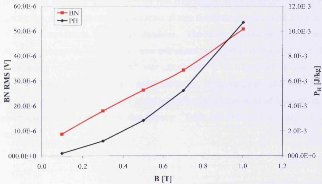
Figure 6.24. Variation of static hysteresis loss, P_H , and rms Barkhausen noise, BN RMS, with peak magnetic flux density, B , at 50 Hz magnetising frequency, for 0.1 mm thick non-oriented electrical steel with 5.5%Si, measured with the double B-coil sensor (S6-NO)
