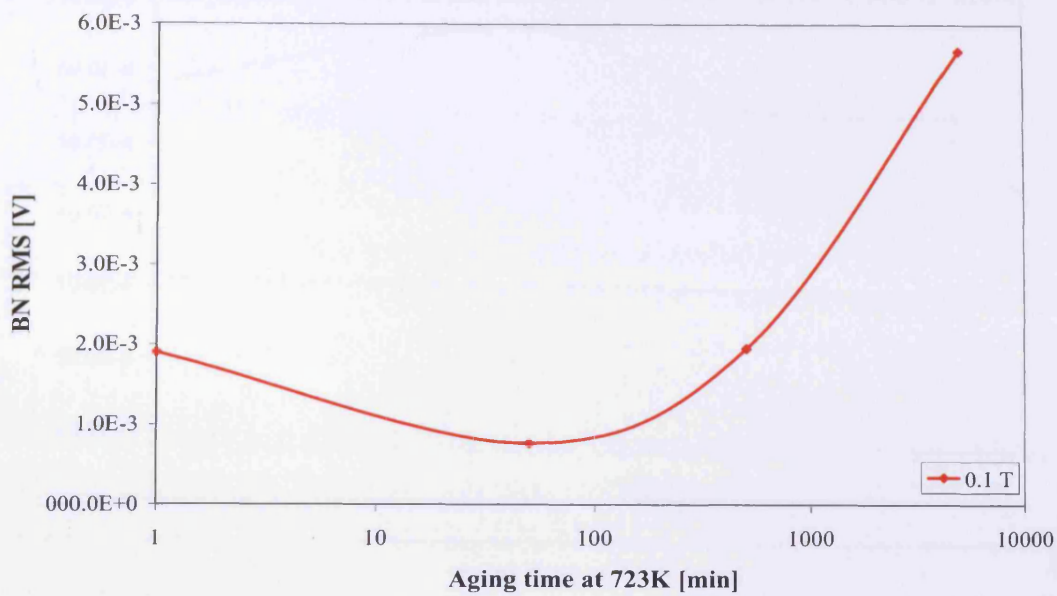
Figure 7.12. Variation of rms Barkhausen noise, BN RMS, with aging time at 723K, at 0.1 T peak flux density, at 50 Hz magnetising frequency, for Charpy shaped thermally aged iron copper samples, of 10% rolling reduction, measured with the double B-coil sensor
