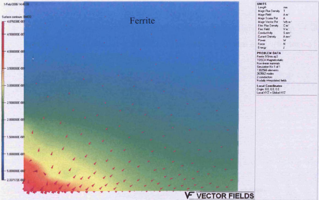
Figure 4.50. Flux density distribution in the ferrite core
