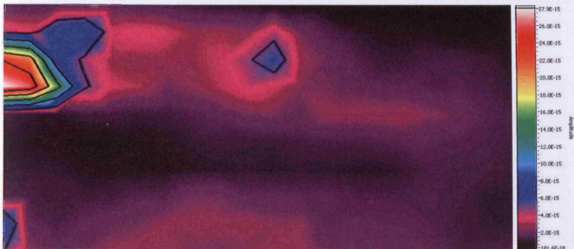
Figure 6.57. Surface scan of kurtosis Barkhausen noise, area scanned 40\text{ mm} \times 20\text{ mm} , at 1.0 T magnetic flux density, at 25 Hz magnetising frequency, for coated 3%Si sample, measured with the ferrite sensor, with step scan of 2 mm
