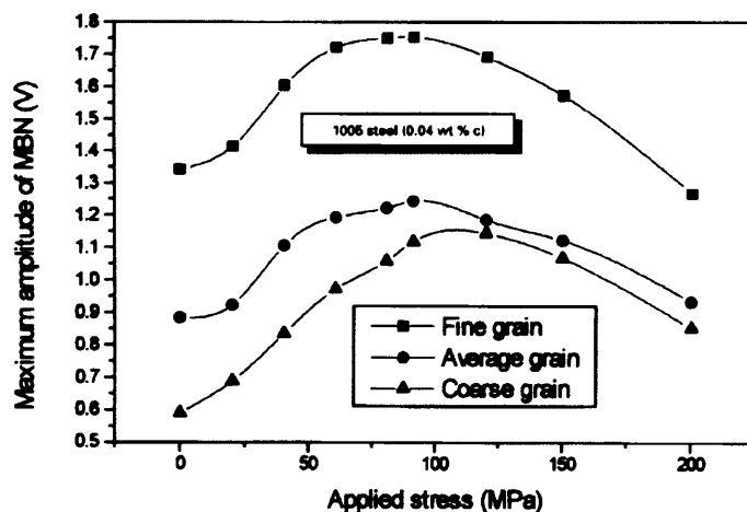
Figure 3.12. Dependence of maximum amplitude of Barkhausen noise (MBN), with applied stress for three different grain sizes ( H=2.13 \times 10^5 A/m) of 1005 carbon steel [3.30]
