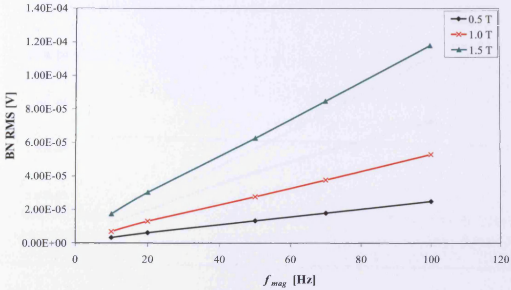
Figure 6.9. Variation of rms Barkhausen noise with magnetising frequency, f_{mag} , at 0.5 T, 1.0 T, 1.5 T magnetic flux density, for grain-oriented electrical steel cut at 0^\circ to the rolling direction, 0.27 mm thick, measured with the double B-coil sensor
