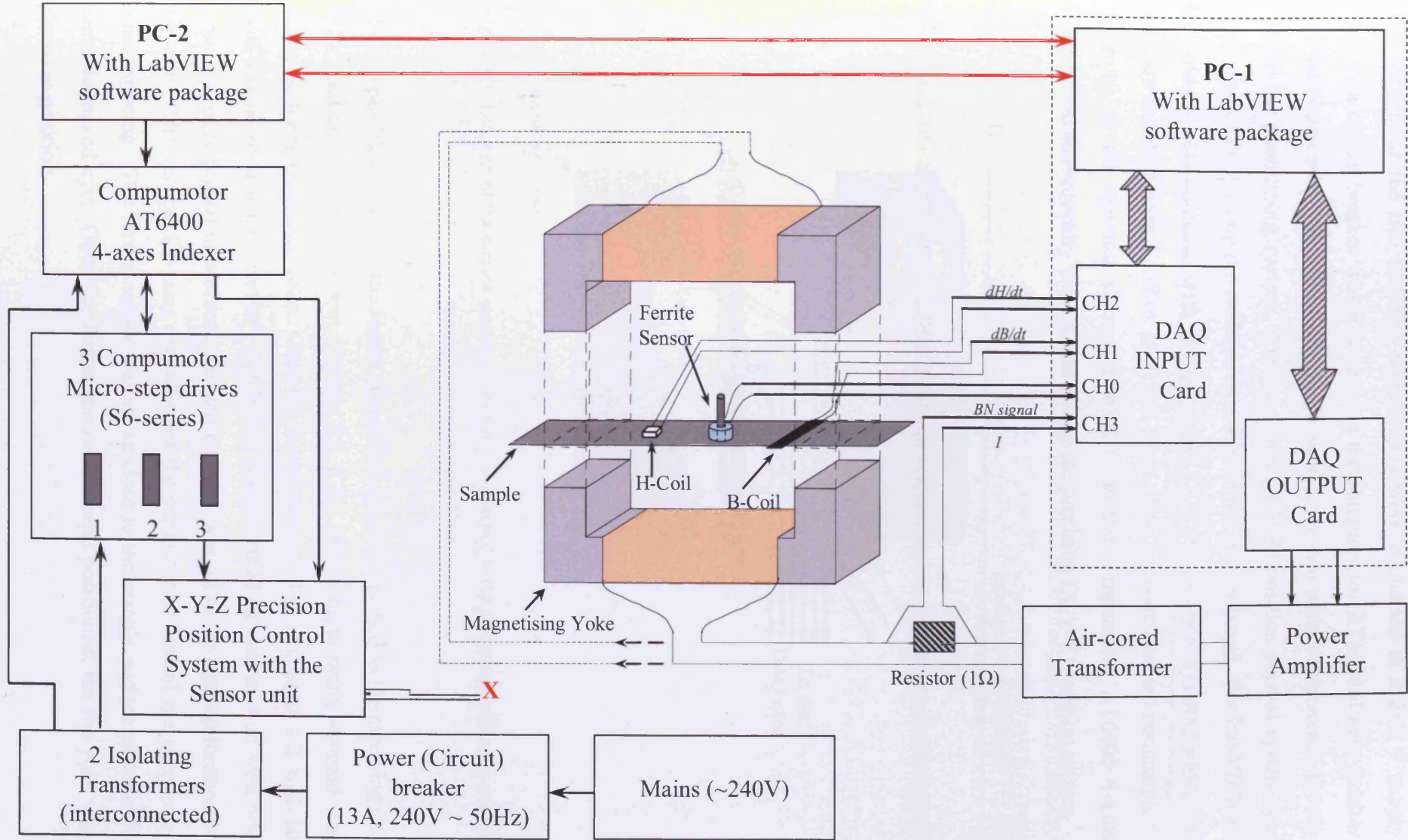
Figure 5.1. Block diagram of the Barkhausen Noise Scanning Measurement System
