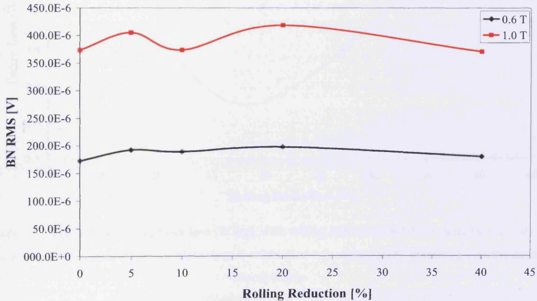
Figure 7.4. Variation of rms Barkhausen noise, BN RMS, with rolling reduction, at 0.6 T, 1.0 T peak flux density, at 50 Hz magnetising frequency, for picture frame shaped cold rolled low carbon steel, measured with the double B-coil sensor
