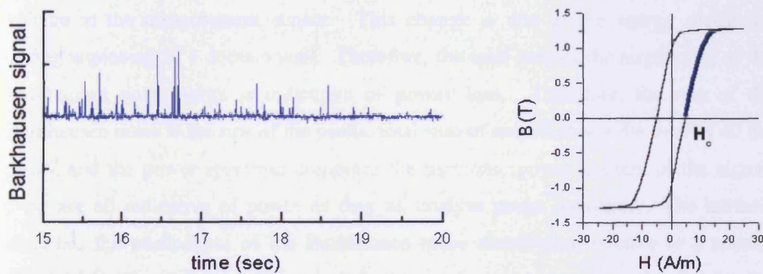
Figure 6.1. Barkhausen noise signal for Co-base amorphous alloy, magnetised at 20 mHz [6.4]
