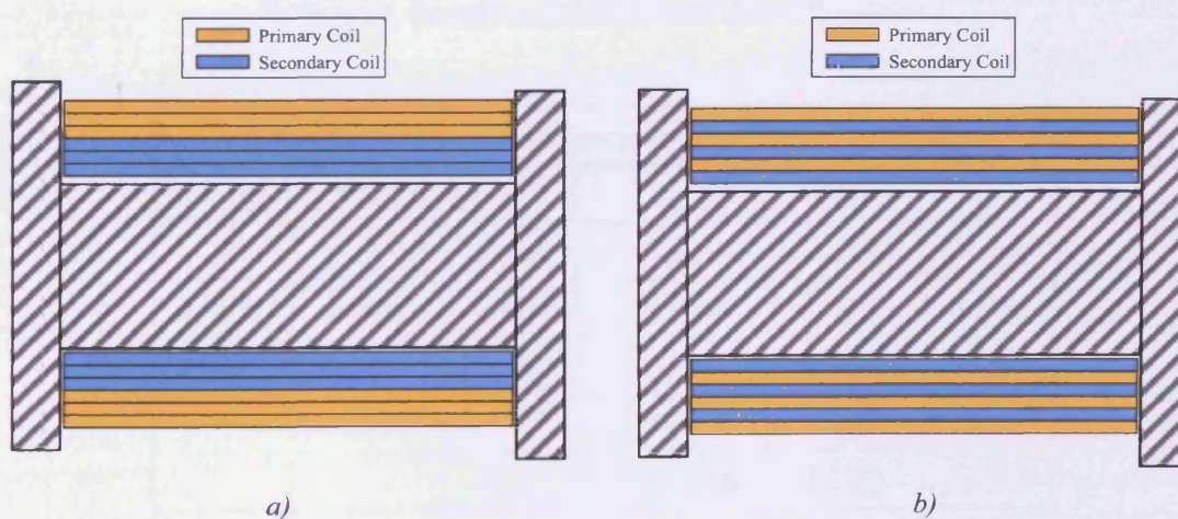
Figure 4.28. Winding configurations of air-cored transformer a) primary winding on the outside and secondary wind on the inside b) inter layered windings with primary and secondary winding layered.
