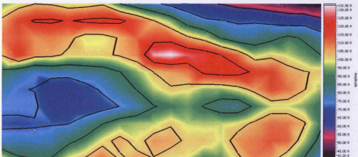
Figure 6.50. Surface scan of power spectrum of Barkhausen noise, area scanned 40 mm \times 20 mm, at 1.0 T magnetic flux density, at 50 Hz magnetising frequency, for coated 3%Si sample, measured with the ferrite sensor, with step scan of 2 mm
