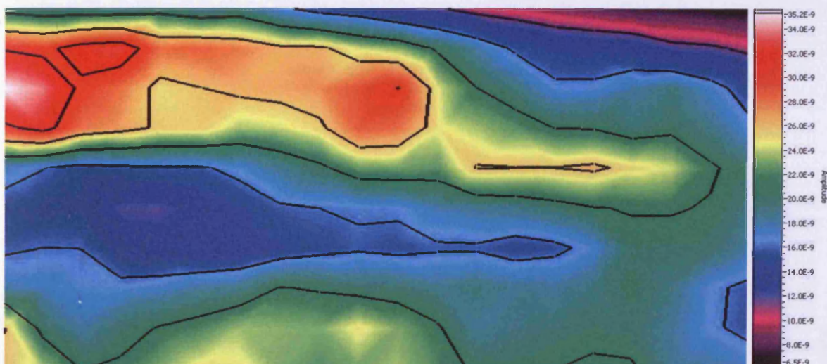
Figure 6.58. Surface scan of power spectrum of Barkhausen noise, area scanned 40\text{ mm} \times 20\text{ mm} , at 1.0 T magnetic flux density, at 25 Hz magnetising frequency, for coated 3%Si sample, measured with the ferrite sensor, with step scan of 2 mm
