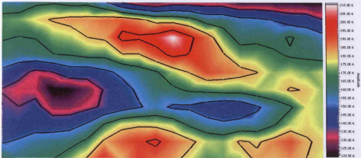
Figure 6.51. Surface scan of rms Barkhausen noise, area scanned 40\text{ mm} \times 20\text{ mm} , at 0.5\text{ T} magnetic flux density, at 50\text{ Hz} magnetising frequency, for coated 3\%Si sample, measured with the ferrite sensor, with step scan of 2\text{ mm}
