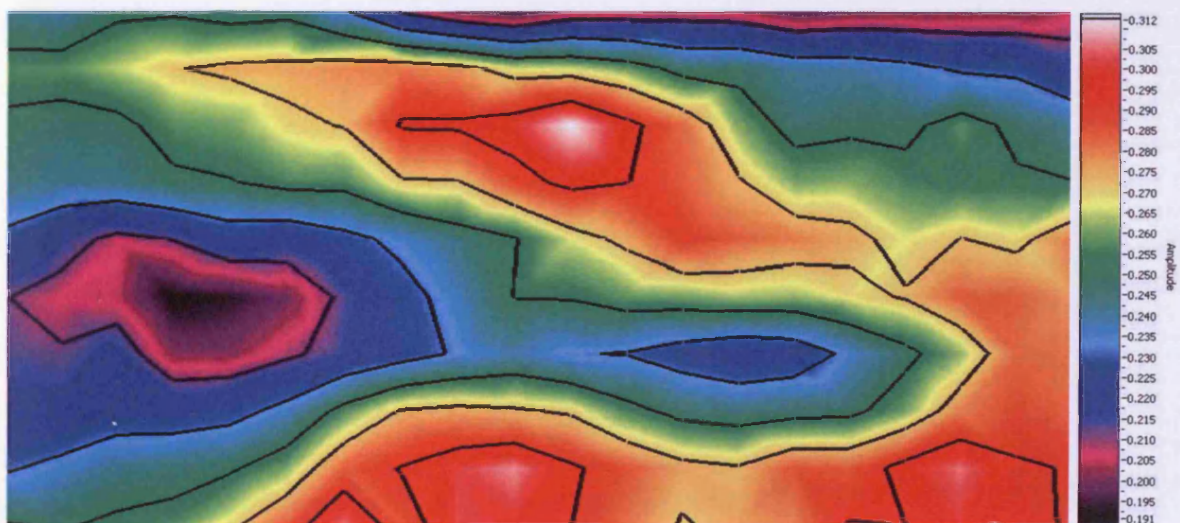
Figure 6.52. Surface scan of total sum of amplitudes of Barkhausen noise, area scanned 40\text{ mm} \times 20\text{ mm} , at 0.5\text{ T} magnetic flux density, at 50\text{ Hz} magnetising frequency, for coated 3\%Si sample, measured with the ferrite sensor, with step scan of 2\text{ mm}
