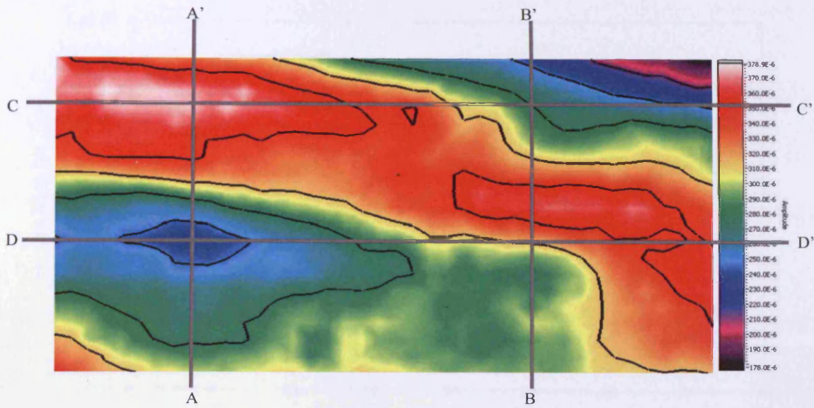
Figure 6.68. Surface scan of rms Barkhausen noise, area scanned 40 mm × 20 mm, at 1.0 T magnetic flux density, at 50 Hz magnetising frequency, for coated 3%Si sample, measured with the ferrite sensor, with step scan of 1 mm, indicating paths A-A', B-B', C-C' and D-D'
