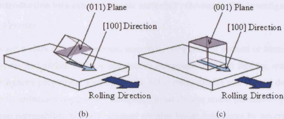
Figure 2.7. Schematic diagram of (a) the magnetocrystalline anisotropy of Fe, (b) cube-on-edge texture and (c) cube texture in grain-oriented silicon steel
