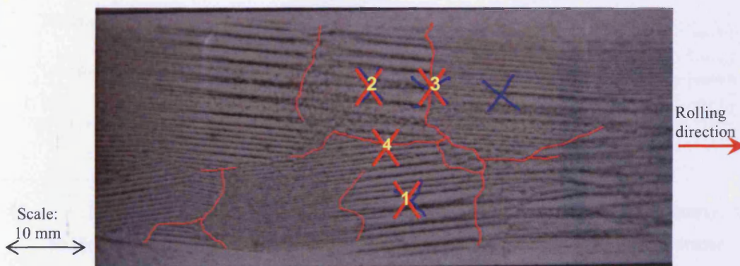
Figure 6.37. Photo of the grains in the coated grain-oriented 3%SiFe electrical steel sample using the magnetic domain viewer. The numbers indicate the location where the ferrite sensor was placed for measurement of Barkhausen noise (position 1 & 2 are in the centre of a grain and position 3 & 4 are on the grain boundaries)
