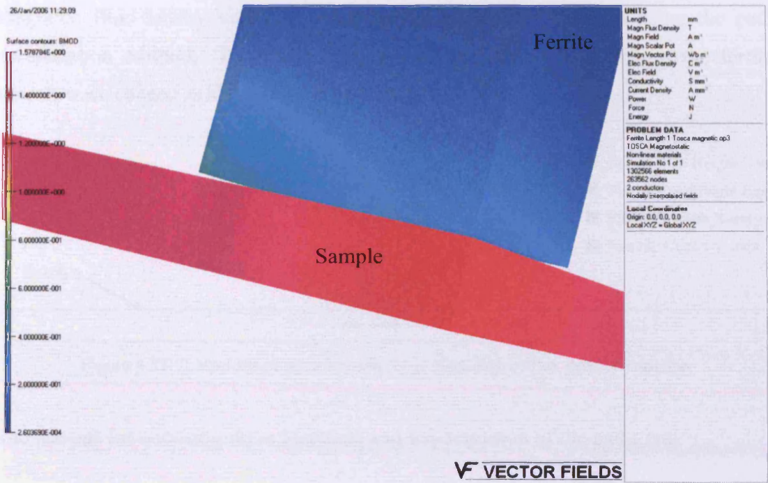
Figure 4.49. Ferrite sensor on sample, expanded image
