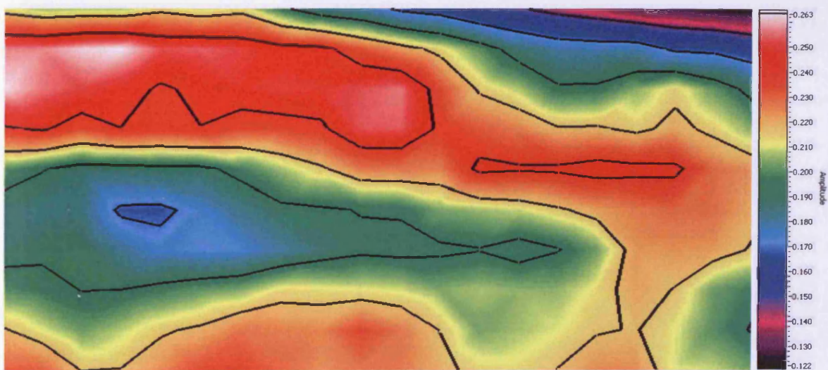
Figure 6.56. Surface scan of total sum of amplitudes of Barkhausen noise, area scanned 40\text{ mm} \times 20\text{ mm} , at 1.0 T magnetic flux density, at 25 Hz magnetising frequency, for coated 3%Si sample, measured with the ferrite sensor, with step scan of 2 mm
