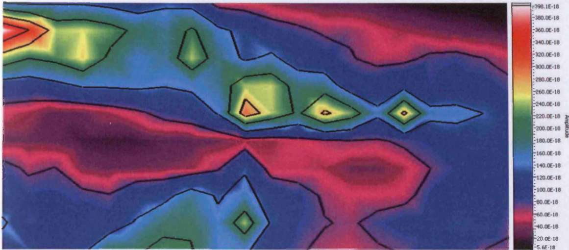
Figure 6.61. Surface scan of kurtosis Barkhausen noise, area scanned 40\text{ mm} \times 20\text{ mm} , at 0.5\text{ T} magnetic flux density, at 25\text{ Hz} magnetising frequency, for coated 3\%\text{Si} sample, measured with the ferrite sensor, with step scan of 2\text{ mm}
