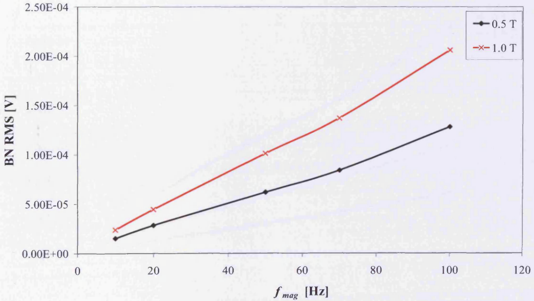
Figure 6.10. Variation of rms Barkhausen noise with magnetising frequency, f_{mag} , at 0.5 T, 1.0 T magnetic flux density, for grain-oriented electrical steel cut at 55^\circ to the rolling direction, 0.27 mm thick, measured with the double B-coil sensor
