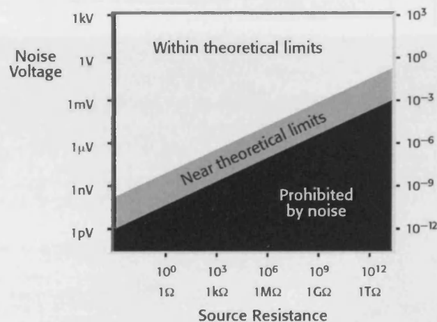
Figure 4.9. Theoretical limits of voltage measurements [4.4]
