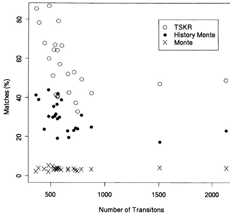
Figure 6.9: Match rate of predicted states to those observed
