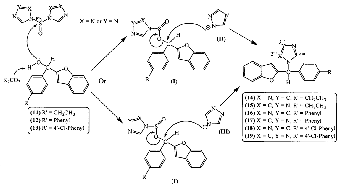
Scheme 3.8. The mechanism of the synthesis of substituted 1- and 4-[(benzo[ b ]furan-2-yl)phenylmethyl]triazoles ( 14 – 19 ). Reaction conditions: 1,2,4-triazole, SOCl 2 , acetonitrile, 10 °C, 1h then add K 2 CO 3 , carbinol compound ( 11, 12 or 13 ), r.t., 4 – 6 days.
