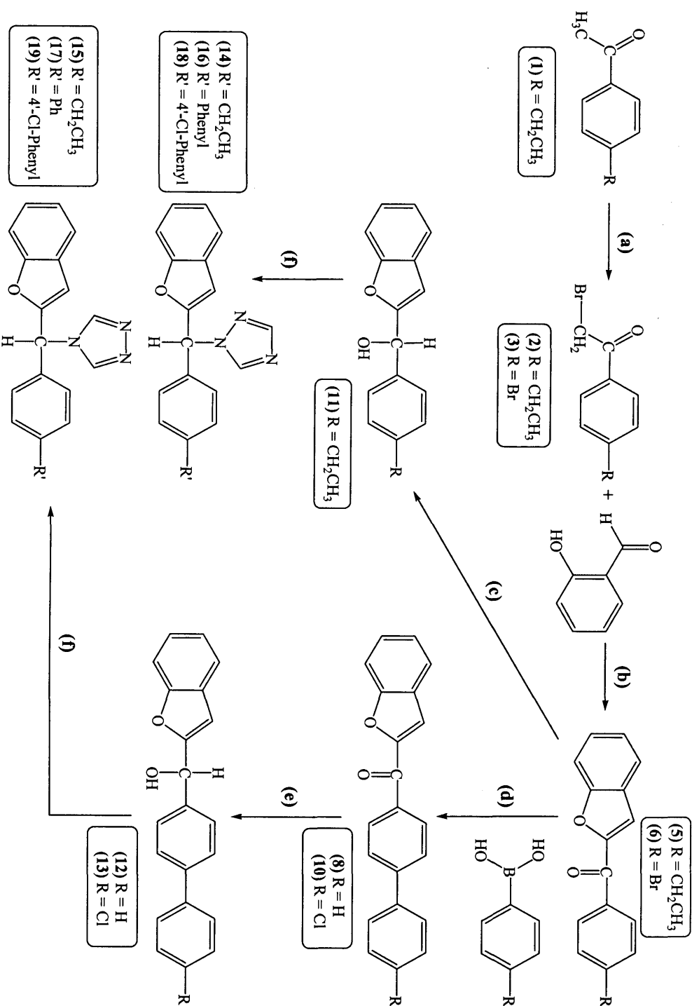
Scheme 3.1. General reaction scheme for the synthesis of substituted 1- and 4-[(benzofuran-2-yl)phenyl]methyl]triazoles. Reagents and conditions: (a) \text{Br}_2 , \text{AlCl}_3 , \text{THF} , 0^\circ\text{C} , 3.5 h. (b) (i) \text{NaH} , \text{DMF} , 80^\circ\text{C} , 2.5 h, (ii) \text{NaOMe} , 80^\circ\text{C} , 1.5 h. (c) and (e) \text{NaBH}_4 , 1,4-dioxane, 6 h. (d) (i) phenylboronic acid or 4-chlorophenylboronic acid, \text{Pd}(\text{PPh}_3)_4 , toluene, 100^\circ\text{C} , 4 h (ii) \text{H}_2\text{O}_2 , room temperature, 1 h. (f) (i) 1,2,4-triazole, thionyl chloride, acetonitrile, 10^\circ\text{C} , 1 h, (ii) \text{K}_2\text{CO}_3 , room temperature, 4–6 days.
