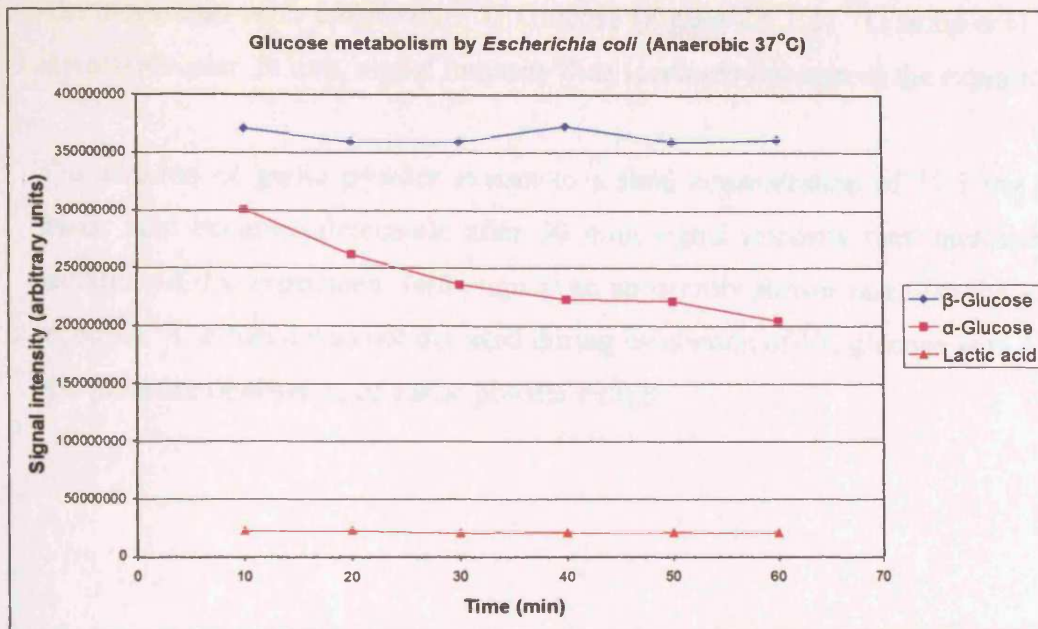
Figure 8.5.1.0 Metabolism of 13 C glucose by E. coli (anaerobic conditions at 37°C in nutrient broth). Trends shown here are typical of 2 independent repeats.
