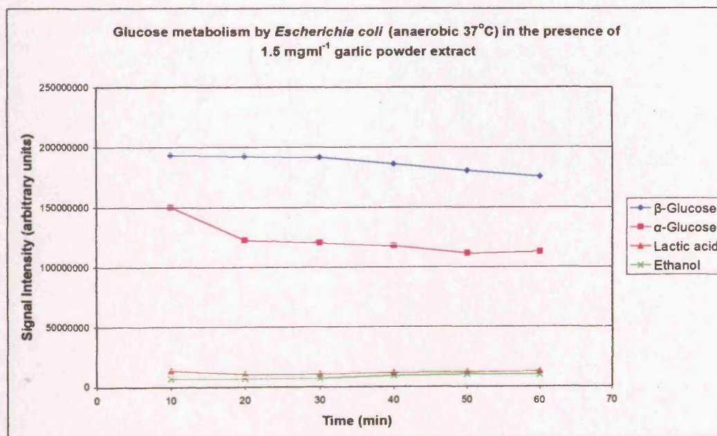
Figure 8.5.1.1 Metabolism of 13 C glucose by E. coli in the presence of 1.5 mg ml -1 garlic extract (anaerobic conditions at 37°C in nutrient broth). Trends shown here are typical of 2 independent repeats.
