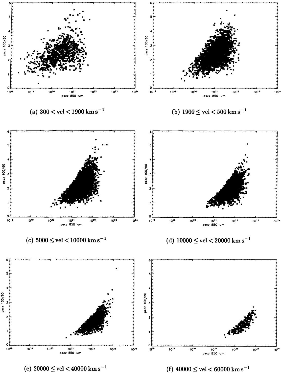
Figure 5.11: PSCz sample: 100–60 \mu\text{m} colour versus extrapolated 850 \mu\text{m} luminosity for the PSCz sample selected in this work, plotted for different velocity ranges.
