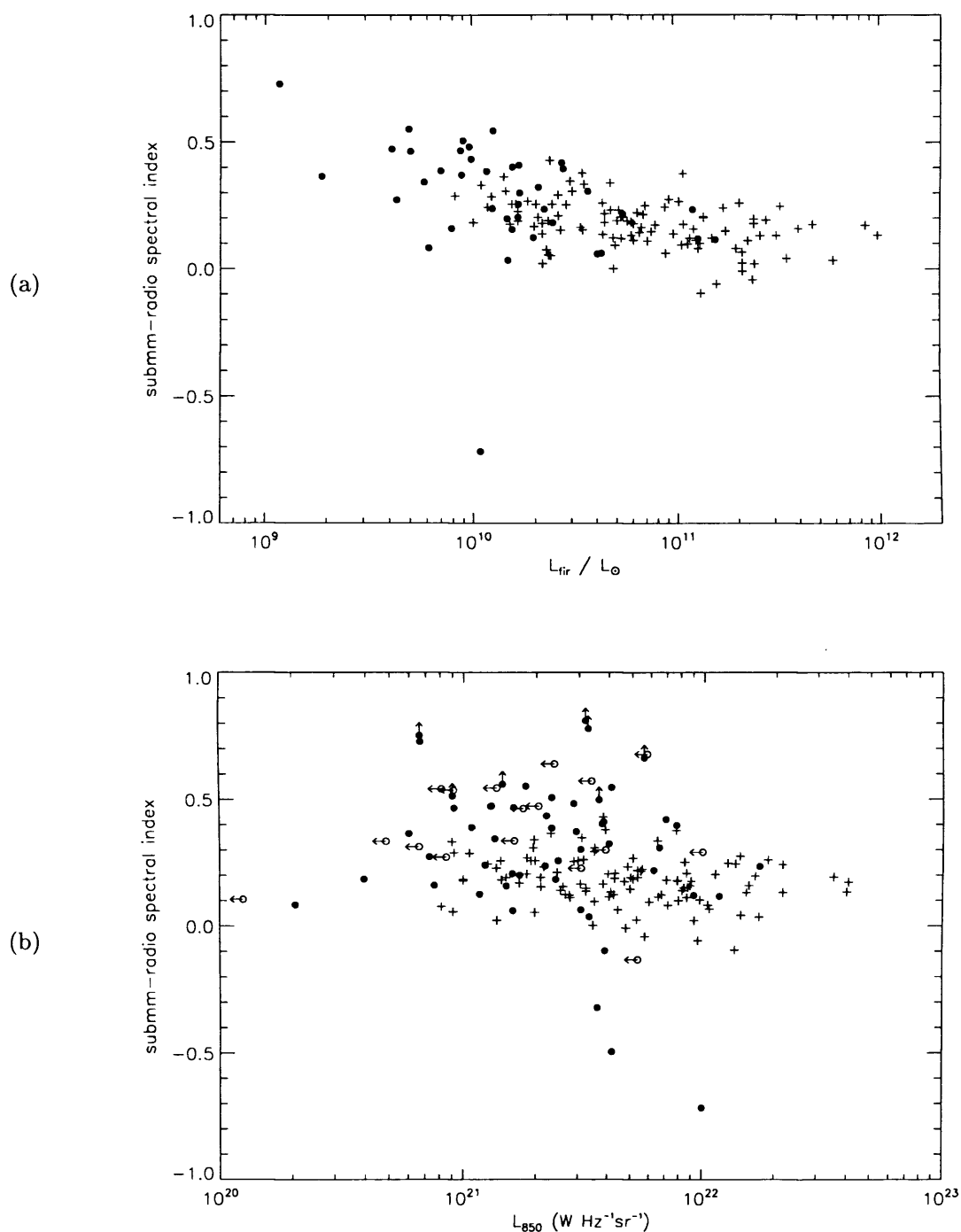
Figure 6.6: \alpha_{1.4}^{850} versus (a) FIR luminosity and (b) 850\ \mu\text{m} luminosity, for the OS and IRS samples. Filled points indicated objects detected at 850\ \mu\text{m} while open points represent the non-detections at 850\ \mu\text{m} . The IRS galaxies are plotted as cross symbols.
