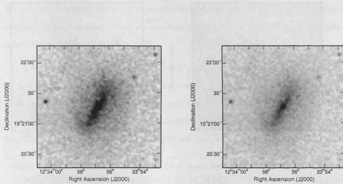
Figure 3.7: IC 800. Clockwise from top left: DSS IR (high contrast), DSS IR (low contrast).
