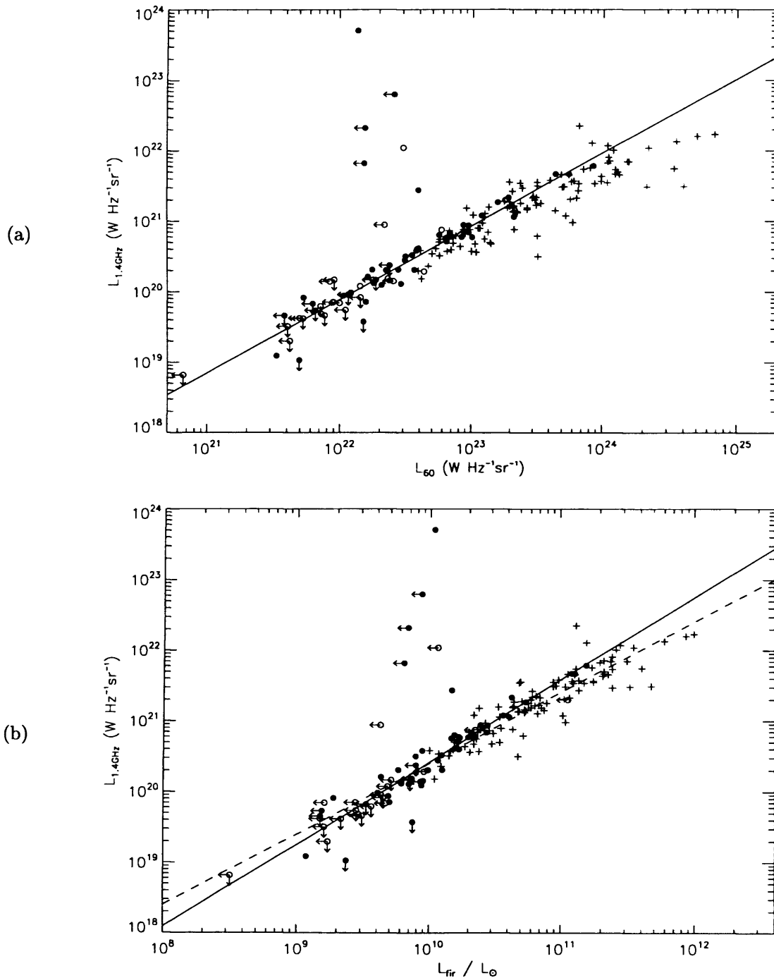
Figure 6.4: 1.4 GHz luminosity versus (a) 60 \mu\text{m} luminosity and (b) FIR luminosity for the OS and IRS samples (circles and crosses respectively; for the OS galaxies filled circles indicate those detected at 850 \mu\text{m} while open circles indicate the non-detections at 850 \mu\text{m} ). The solid lines show the linear fits to the OS data. In (a) the slope is unity and in (b) it is slightly greater than unity; the dashed line indicates a slope of unity for comparison. The 7 OS outliers which have excess 1.4 GHz emission relative to this correlation are mainly ellipticals (NGC6166, NGC6137, NGC6146, UGC7115 and NGC6173; the other two outliers are NGC6185 and NGC7653).
