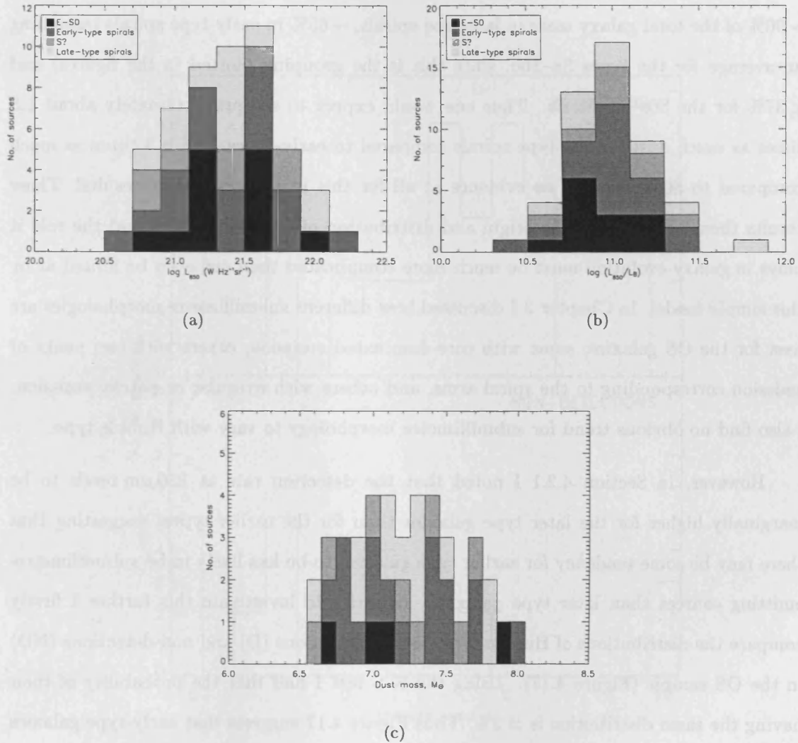
Figure 4.16: Distribution of (a) 850 \mu\text{m} luminosity, (b) 850 \mu\text{m} luminosity / optical blue luminosity, and (c) dust masses, for the Optically-Selected SLUGS (as listed in Chapter 3 Table 3.4, with different Hubble types (as given in the LEDA database according to the RC2 code, and listed in Chapter 3 Table 3.1) indicated by different shaded regions: E-S0( t=-5 to 0), Early-type spirals( t=1 to 4), S?( t=5 ), Late-type spirals( t=6 to 10)).
