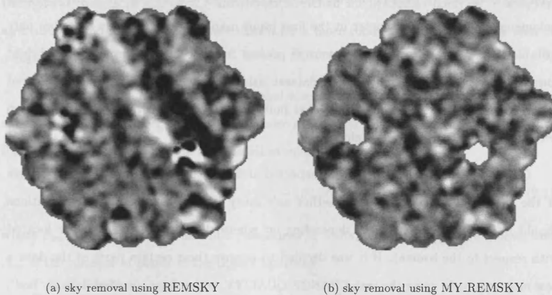
Figure 2.5: An example of the removal of a ‘stripey sky’, in this case for UGC7157. In (a) the sky was removed using REMSKY, leaving a ‘stripey sky’. In (b) the sky was removed using MY.REMSKY – the ‘stripey sky’ is removed.
