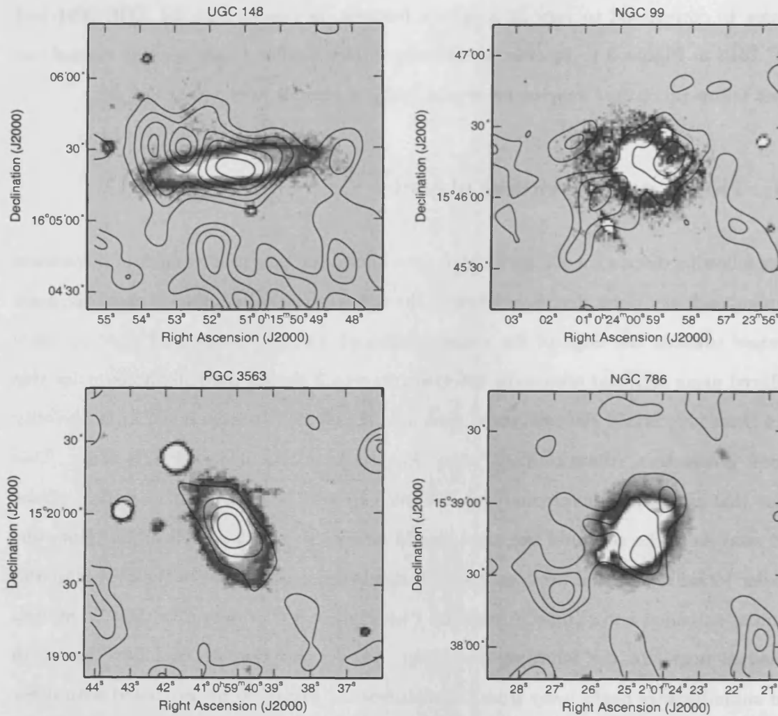
Figure 3.1: The optically-selected SLUGS: 850 \mu\text{m} SCUBA S/N maps (produced as described in Chapter 2 Section 2.9; 1\sigma contours) overlaid onto DSS optical images ( 2' \times 2' , except for NGC 803 and NGC 6155 which are 3' \times 3' ); the point spread function in the SCUBA S/N maps is \sim 19 arcsec (see Chapter 2 Section 2.9). (Optical images are shown here with a contrast that optimises the optical features, however when used as a guide for drawing SCUBA flux measurement apertures a more conservative stretch was applied).
