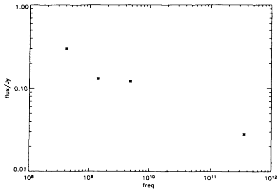
(c) NGC 6146
