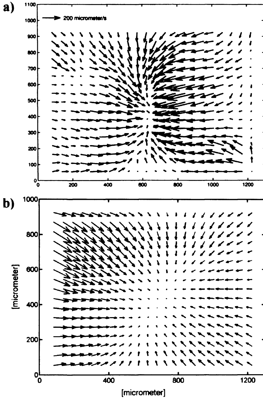
Figure 3.1: PIV maps showing the trajectories followed by 25 μm diameter latex particles towards the central aggregation area in the rectangular ((a); Spengler, 2002) and circular (b) acoustic trap. It is noted that (b) is a qualitative, descriptive map based on observation of radial cell movement towards the axis in a way that did not show preferred pathways as in Figure 3.1a
