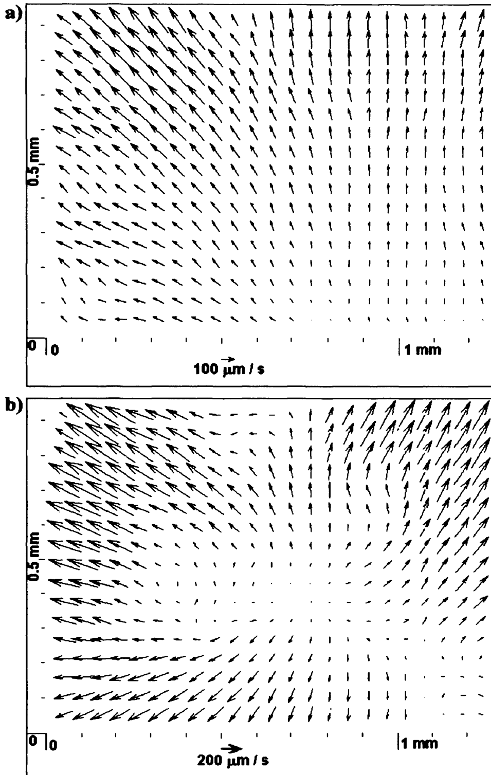
Figure 3.6: PIV analysis of 1 μm diameter latex particles behaviour in the presence of a neural cell suspension at the centre of the trap (a) 1 s after ultrasound initiation and (b) 3 s after ultrasound initiation, when an aggregate has been formed. The presence of the aggregate causes the streaming in the nodal plane to emanate from the centre. The acoustic pressure amplitude was 0.54 MPa.
