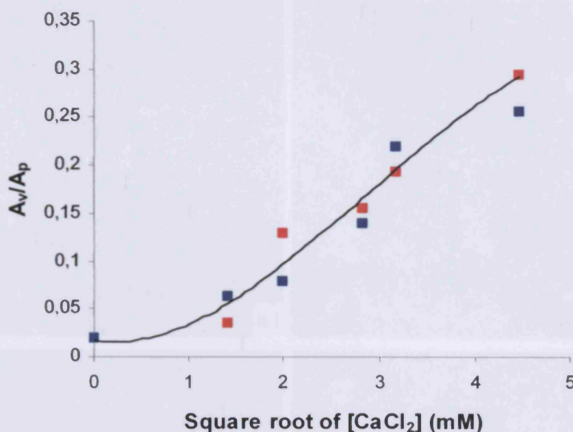
Figure 2.6: [\text{CaCl}_2] dependence of the void index (total void area/total image area) for duplicates of 25 \mu\text{m} latex aggregates. The trend is a third order polynomial best fit to the data.
