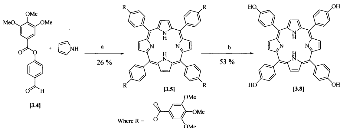
Figure 3.13: Reaction scheme illustrating the use of 3,4,5-trimethoxybenzyl ester as a protecting group for the phenol. Reagents and conditions: (a) propionic acid, reflux, 0.5 h; (b) hydrazine monohydrate, EtOH, reflux.
