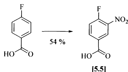
Figure 5.14: Reagents and conditions: potassium nitrate, concentrated sulphuric acid, 130 °C
