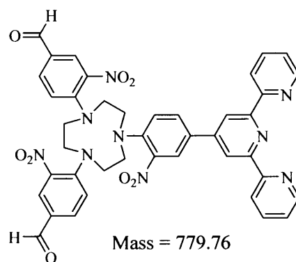
Figure 5.32: Possible structural for the peak observed at 780.5 Da/e.
