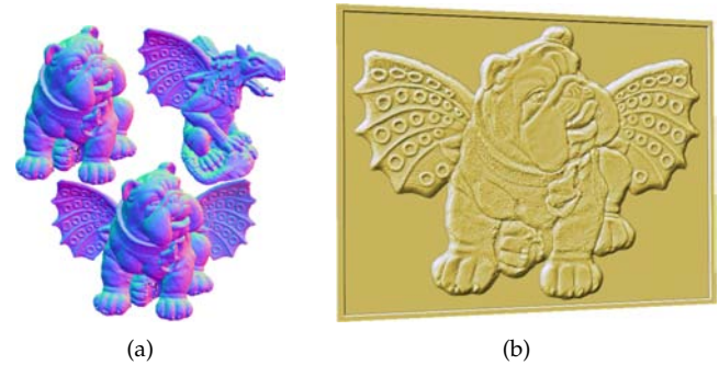
Fig. 15: Bas-relief created by cut-and-paste operations in conjunction with a flip transformation of the wing: (a) a composite normal image created by merging the normal images; and (b) the resulting bas-relief.
