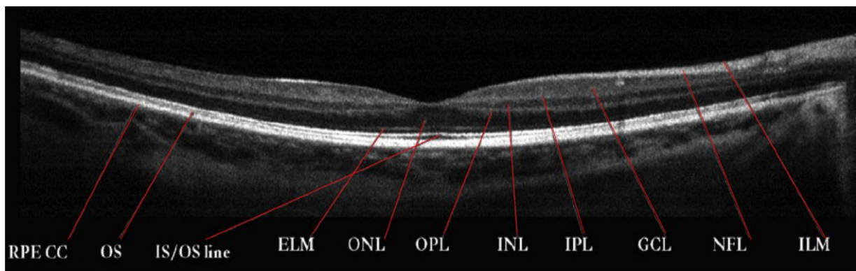
Figure 1.19 OCT of a healthy macular showing the retinal layers. Image from Sheth, Rush and Natarajan (2012). Key: RPE CC, retinal pigment epithelium chorio capillary complex; OS, outer segment; IS, inner segment; ELM, external limiting membrane; ONL, outer nuclear layer; OPL, outer plexiform layer; INL, inner nuclear layer; IPL, inner plexiform layer; GCL, ganglion cell layer; NFL, nerve fiber layer; ILM, internal limiting membrane.
