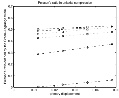
Figure 6: Poisson's ratio computed using (a) the logarithmic and (b) the Green-Lagrange strain vs. the primary (axial) displacement in uniaxial compression.
