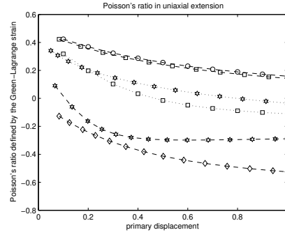
Figure 5: Poisson's ratio computed using (a) the logarithmic and (b) the Green-Lagrange strain vs. the primary (axial) displacement in uniaxial extension.
