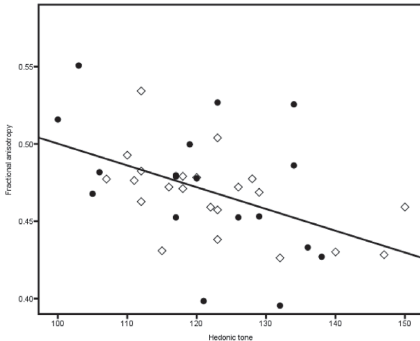
Fig. 2. The negative correlation across the whole sample between mean fractional anisotropy of the left sLMFB and hedonic tone is displayed. ◇, Never depressed; ●, remitted depressed.
