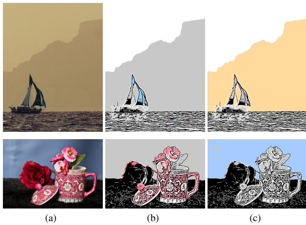
Figure 10: Spot colour and background colourisation. (a) input image, (b) spot colour results using saliency weighted spread criterion, (c) background colourisation.
